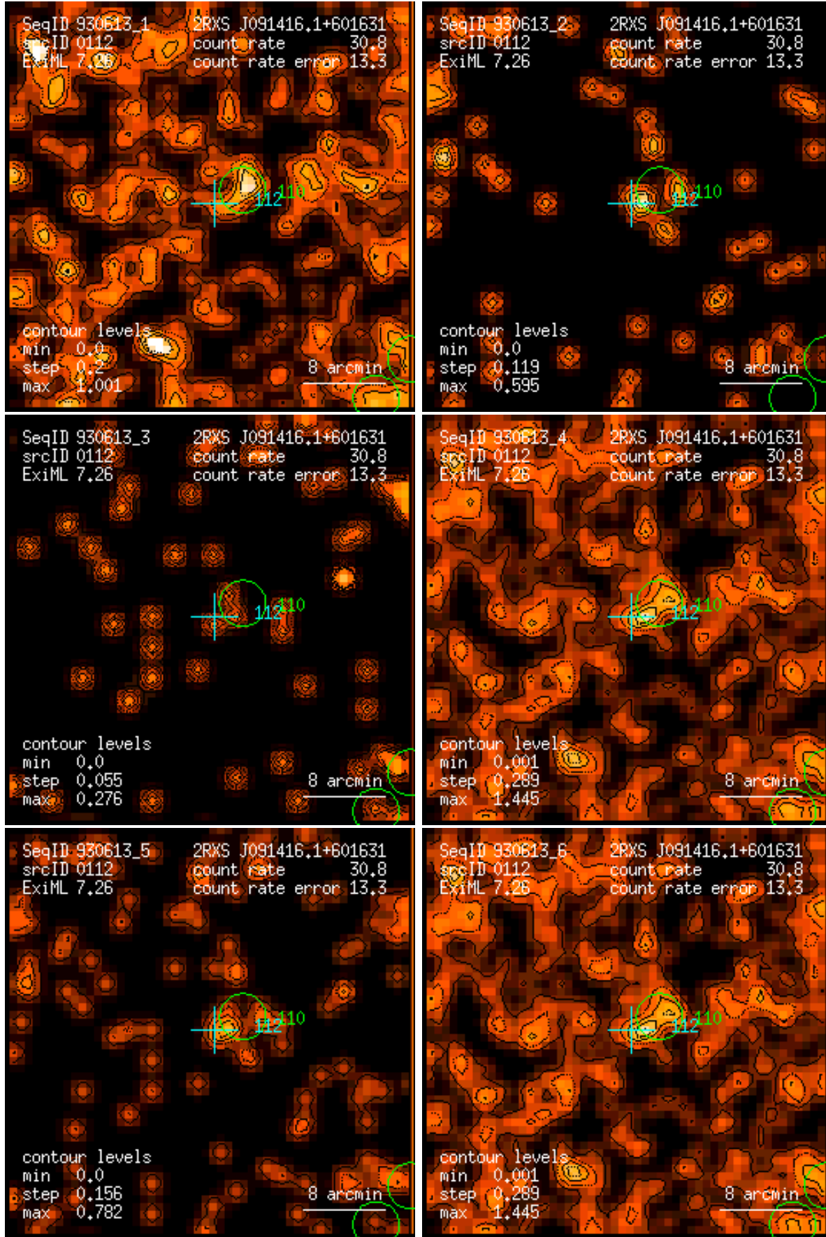
Figure 112: RASS 930613: detection 0112: band rate images, Gaussian filter: (1) PSPC channels 11 – 41, (2) 52 – 90, (3) 91 – 201, (4) 11 – 235, (5) 52 – 201, (6) 11 – 201. Broad band rates in counts/ks. Band rate contour levels in counts/ks/arcmin 2 .
