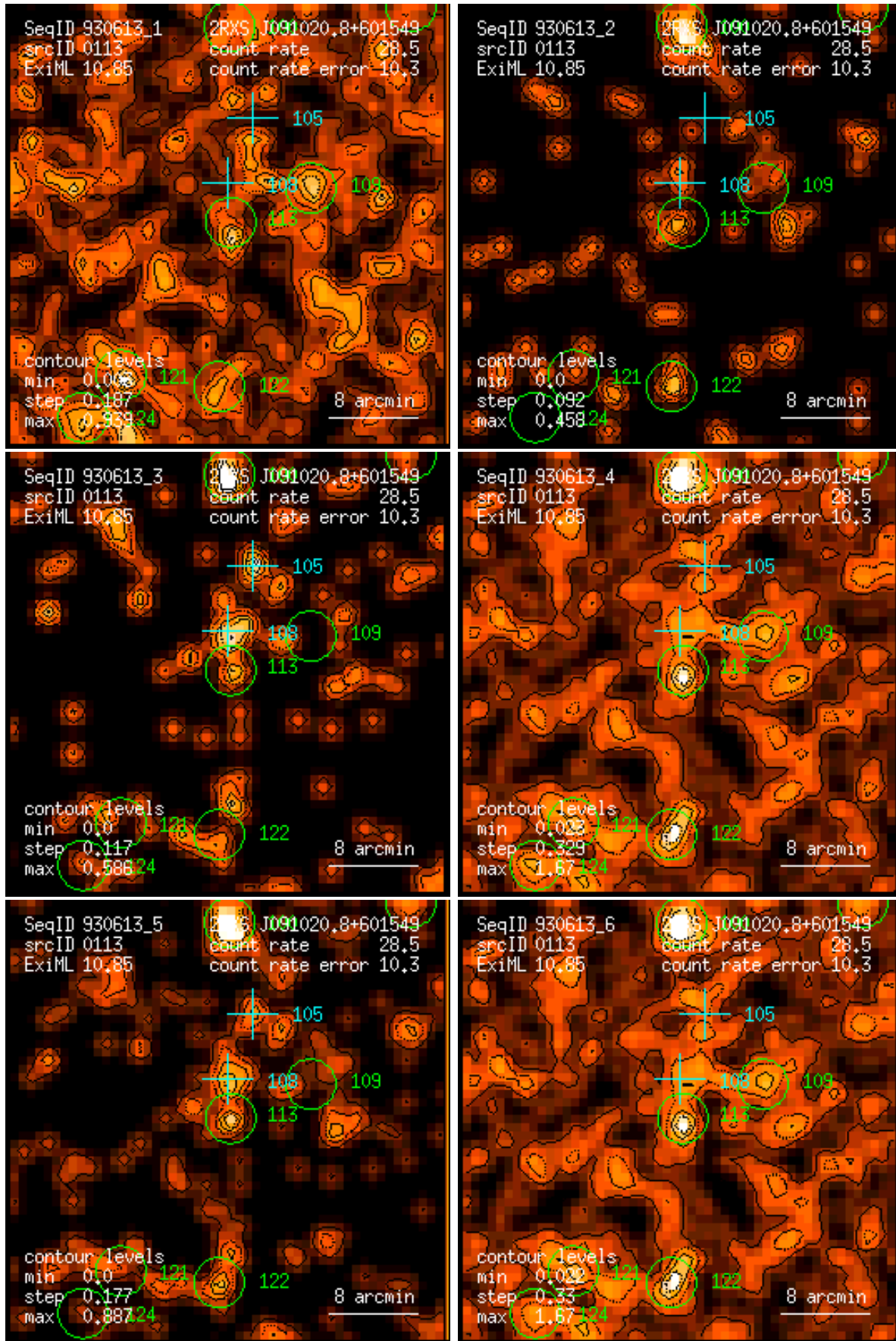
Figure 113: RASS 930613: detection 0113: band rate images, Gaussian filter: (1) PSPC channels 11 – 41, (2) 52 – 90, (3) 91 – 201, (4) 11 – 235, (5) 52 – 201, (6) 11 – 201. Broad band rates in counts/ks. Band rate contour levels in counts/ks/arcmin 2 .
