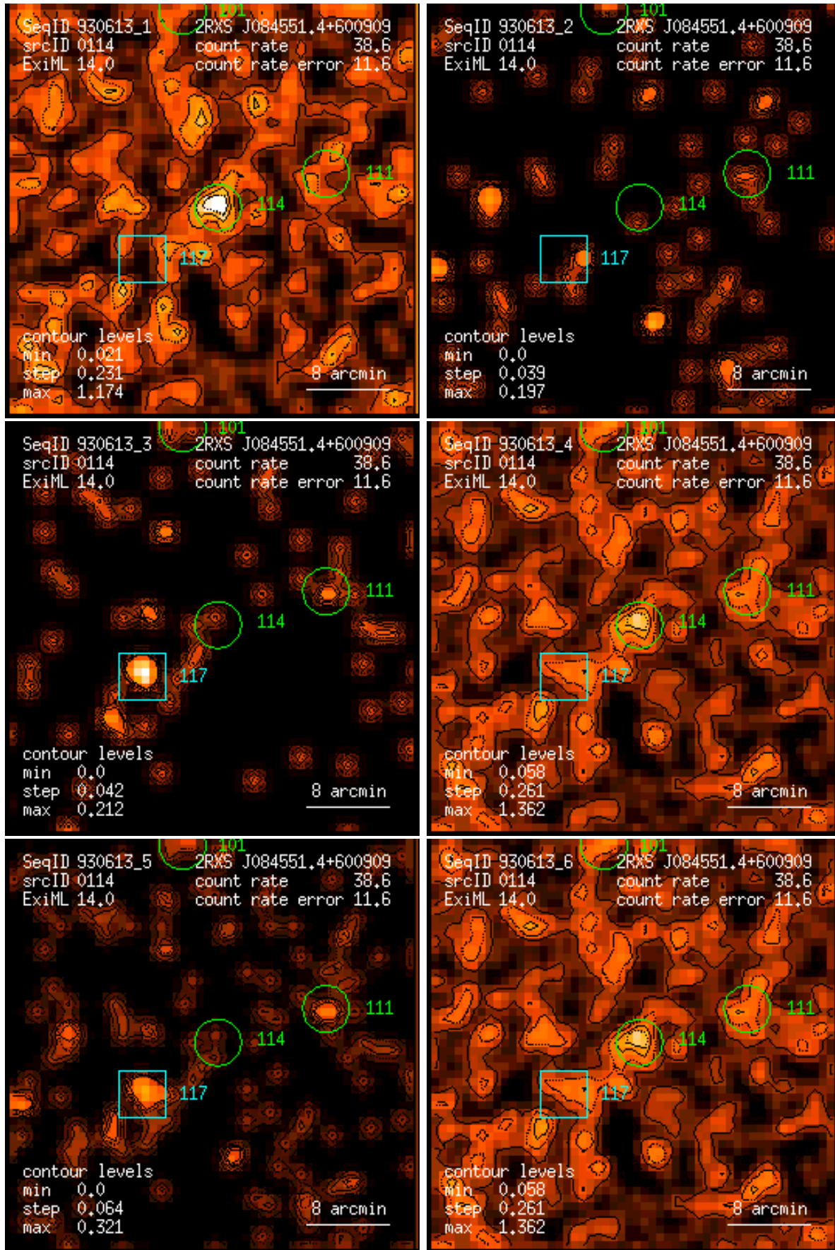
Figure 114: RASS 930613: detection 0114: band rate images, Gaussian filter: (1) PSPC channels 11 – 41, (2) 52 – 90, (3) 91 – 201, (4) 11 – 235, (5) 52 – 201, (6) 11 – 201. Broad band rates in counts/ks. Band rate contour levels in counts/ks/arcmin 2 .
