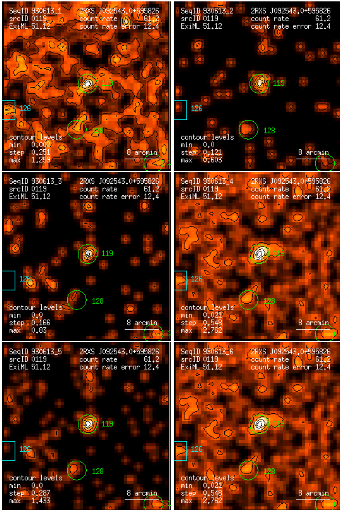
Figure 119: RASS 930613: detection 0119: band rate images, Gaussian filter: (1) PSPC channels 11 – 41, (2) 52 – 90, (3) 91 – 201, (4) 11 – 235, (5) 52 – 201, (6) 11 – 201. Broad band rates in counts/ks. Band rate contour levels in counts/ks/arcmin 2 .
