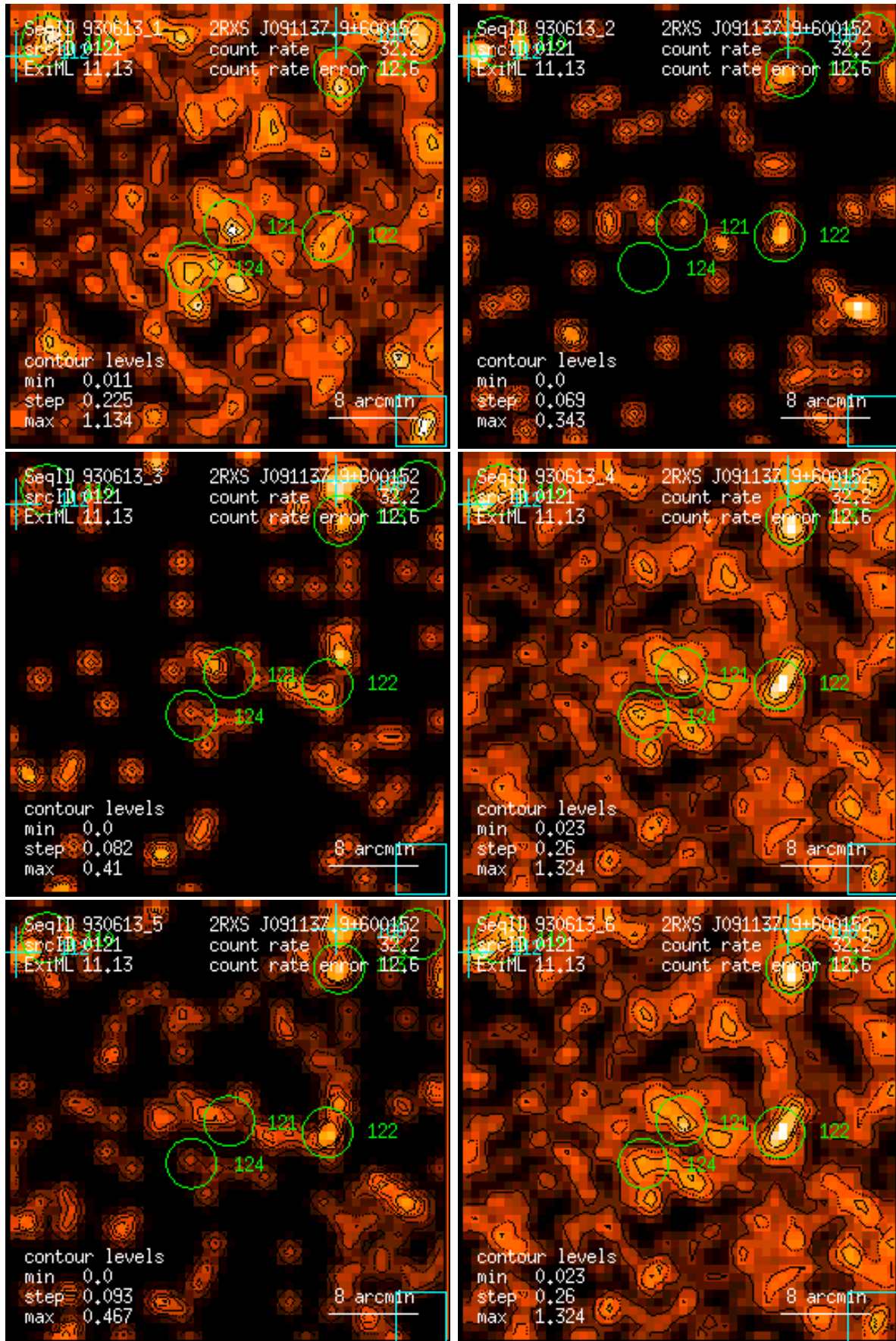
Figure 121: RASS 930613: detection 0121: band rate images, Gaussian filter: (1) PSPC channels 11 – 41, (2) 52 – 90, (3) 91 – 201, (4) 11 – 235, (5) 52 – 201, (6) 11 – 201. Broad band rates in counts/ks. Band rate contour levels in counts/ks/arcmin 2 .
