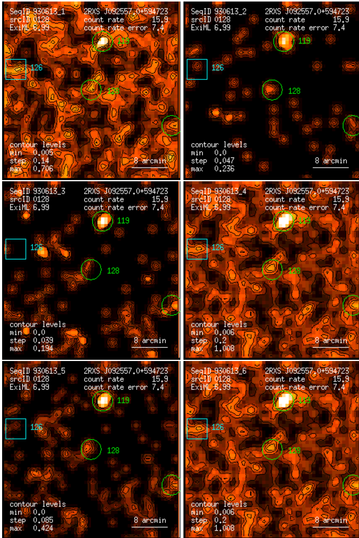
Figure 128: RASS 930613: detection 0128: band rate images, Gaussian filter: (1) PSPC channels 11 – 41, (2) 52 – 90, (3) 91 – 201, (4) 11 – 235, (5) 52 – 201, (6) 11 – 201. Broad band rates in counts/ks. Band rate contour levels in counts/ks/arcmin 2 .
