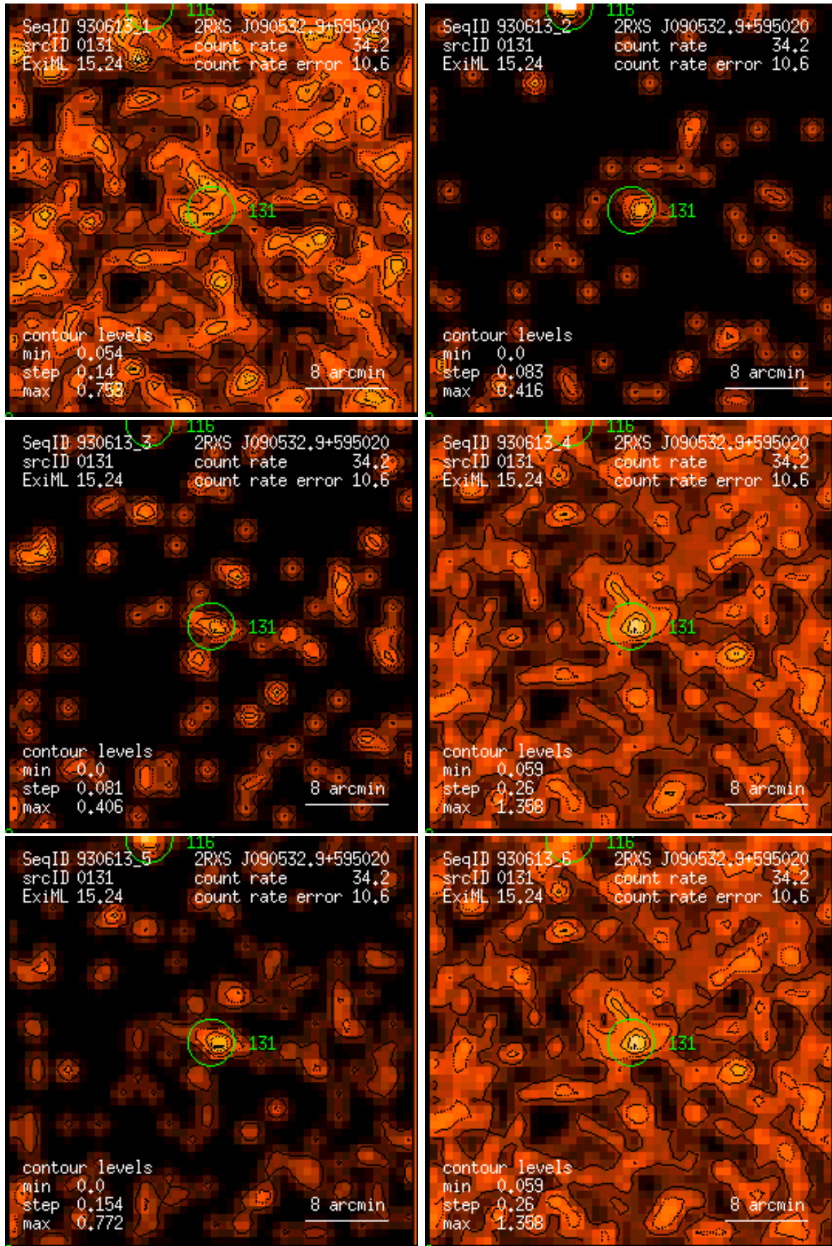
Figure 131: RASS 930613: detection 0131: band rate images, Gaussian filter: (1) PSPC channels 11 – 41, (2) 52 – 90, (3) 91 – 201, (4) 11 – 235, (5) 52 – 201, (6) 11 – 201. Broad band rates in counts/ks. Band rate contour levels in counts/ks/arcmin 2 .
