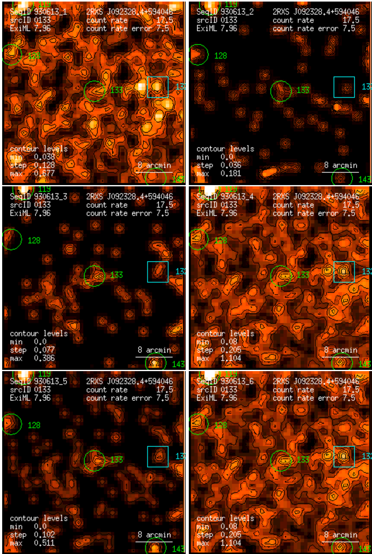
Figure 133: RASS 930613: detection 0133: band rate images, Gaussian filter: (1) PSPC channels 11 – 41, (2) 52 – 90, (3) 91 – 201, (4) 11 – 235, (5) 52 – 201, (6) 11 – 201. Broad band rates in counts/ks. Band rate contour levels in counts/ks/arcmin 2 .
