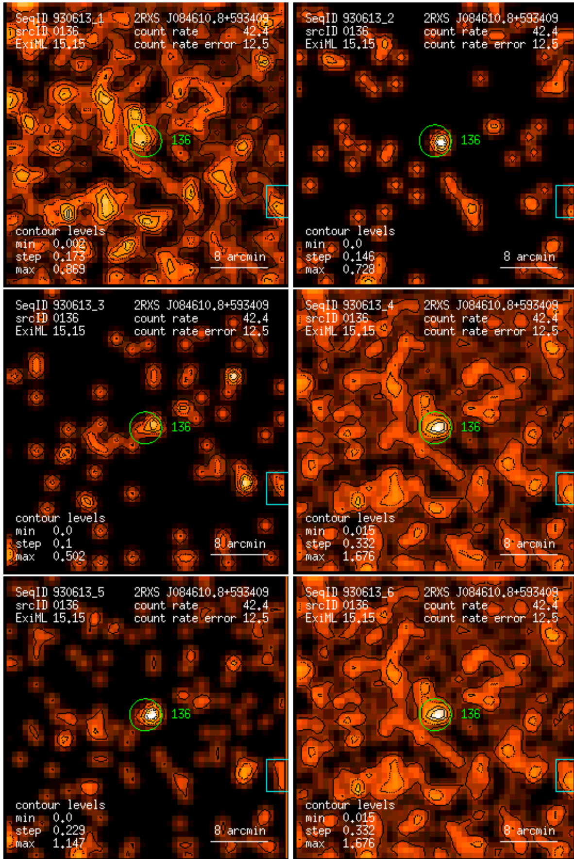
Figure 136: RASS 930613: detection 0136: band rate images, Gaussian filter: (1) PSPC channels 11 – 41, (2) 52 – 90, (3) 91 – 201, (4) 11 – 235, (5) 52 – 201, (6) 11 – 201. Broad band rates in counts/ks. Band rate contour levels in counts/ks/arcmin 2 .
