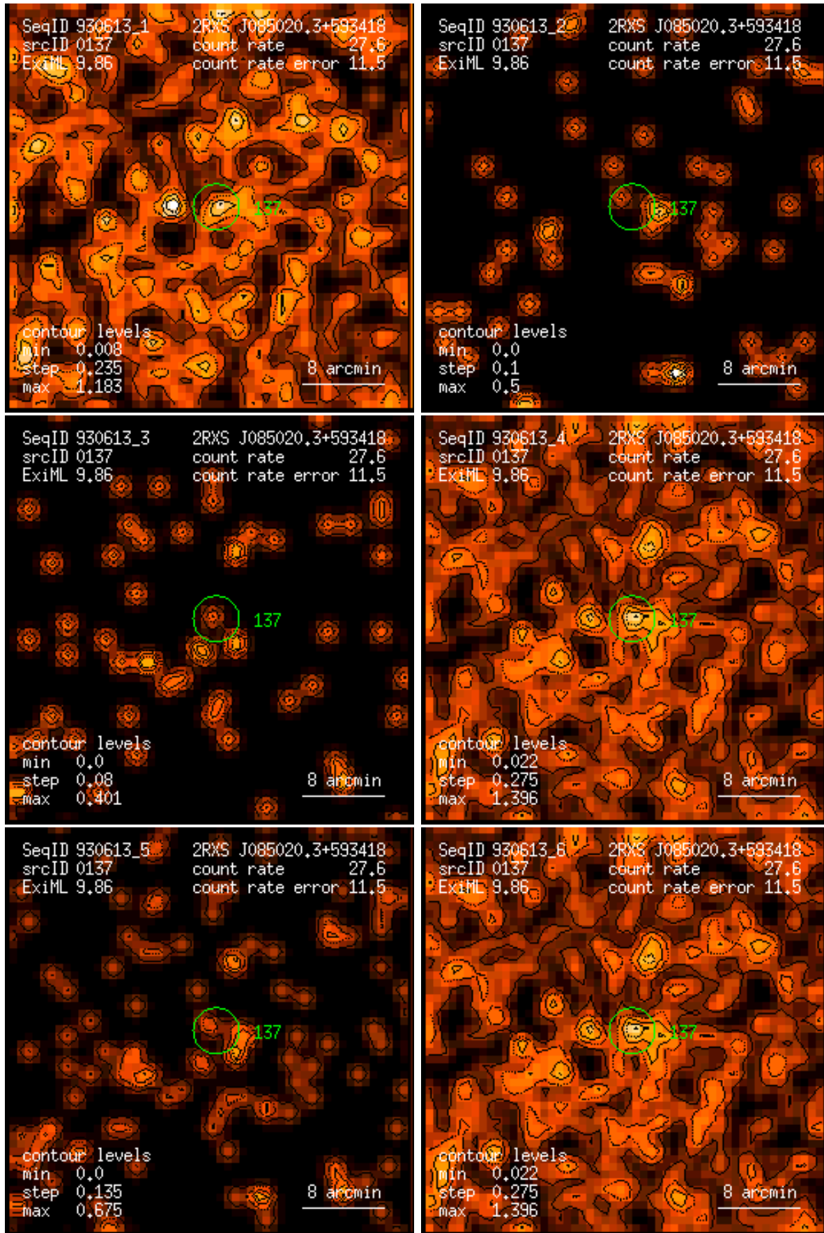
Figure 137: RASS 930613: detection 0137: band rate images, Gaussian filter: (1) PSPC channels 11 – 41, (2) 52 – 90, (3) 91 – 201, (4) 11 – 235, (5) 52 – 201, (6) 11 – 201. Broad band rates in counts/ks. Band rate contour levels in counts/ks/arcmin 2 .
