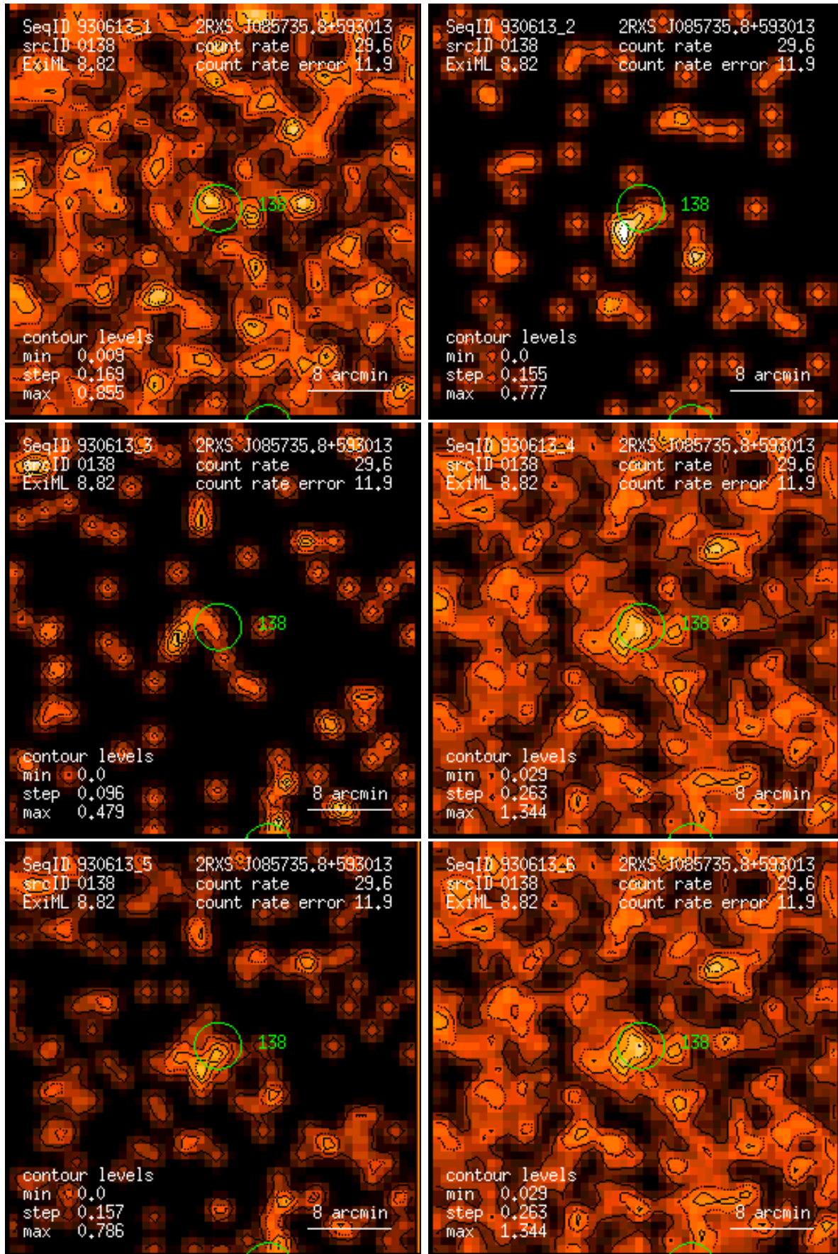
Figure 138: RASS 930613: detection 0138: band rate images, Gaussian filter: (1) PSPC channels 11 – 41, (2) 52 – 90, (3) 91 – 201, (4) 11 – 235, (5) 52 – 201, (6) 11 – 201. Broad band rates in counts/ks. Band rate contour levels in counts/ks/arcmin 2 .
