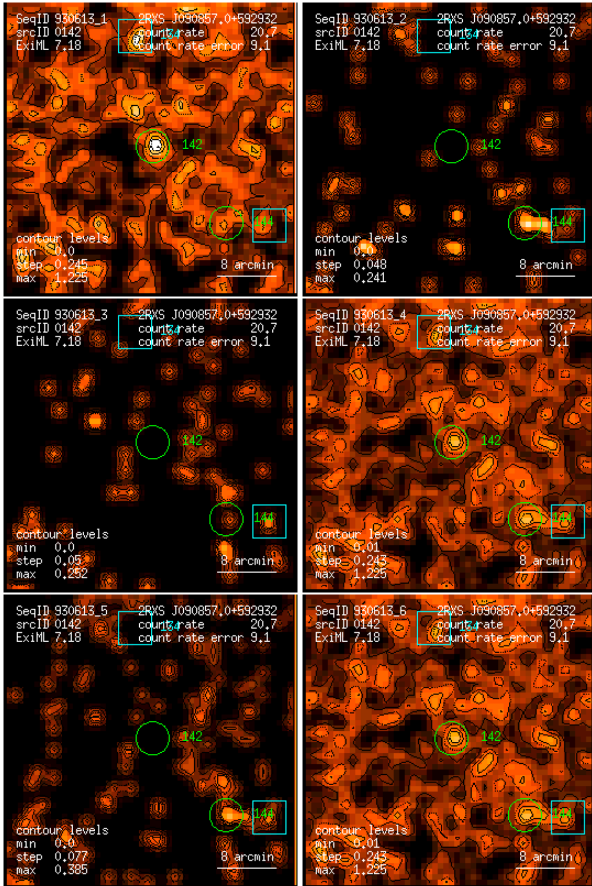
Figure 142: RASS 930613: detection 0142: band rate images, Gaussian filter: (1) PSPC channels 11 – 41, (2) 52 – 90, (3) 91 – 201, (4) 11 – 235, (5) 52 – 201, (6) 11 – 201. Broad band rates in counts/ks. Band rate contour levels in counts/ks/arcmin 2 .
