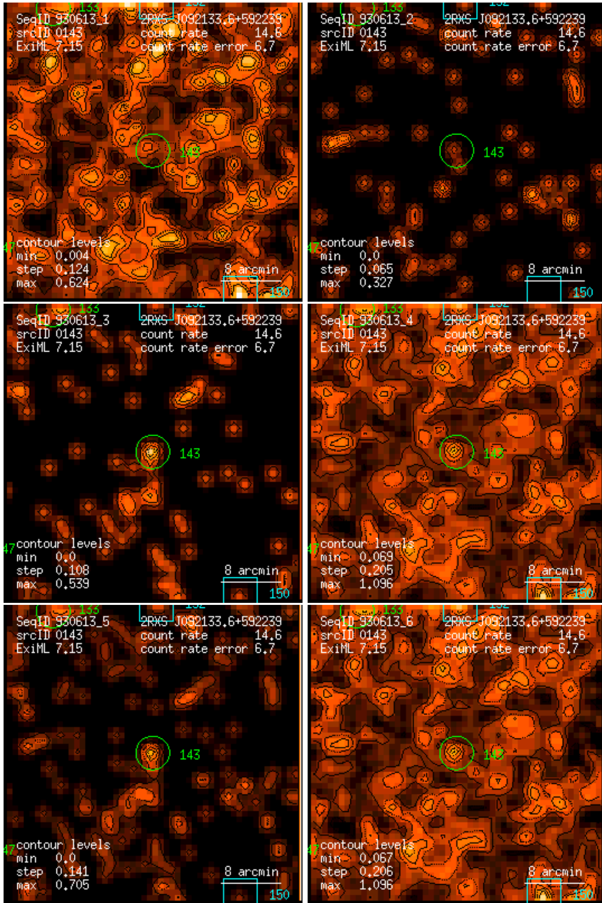
Figure 143: RASS 930613: detection 0143: band rate images, Gaussian filter: (1) PSPC channels 11 – 41, (2) 52 – 90, (3) 91 – 201, (4) 11 – 235, (5) 52 – 201, (6) 11 – 201. Broad band rates in counts/ks. Band rate contour levels in counts/ks/arcmin 2 .
