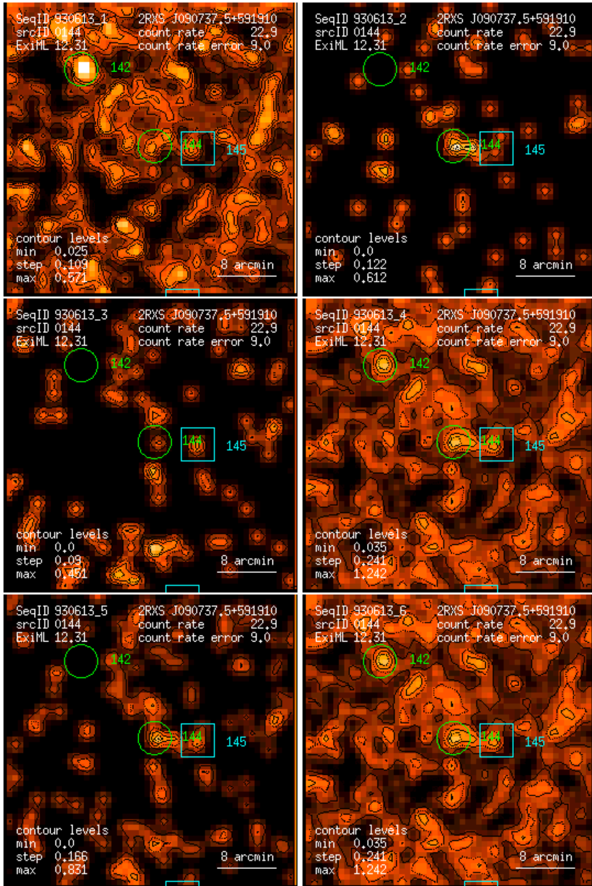
Figure 144: RASS 930613: detection 0144: band rate images, Gaussian filter: (1) PSPC channels 11 – 41, (2) 52 – 90, (3) 91 – 201, (4) 11 – 235, (5) 52 – 201, (6) 11 – 201. Broad band rates in counts/ks. Band rate contour levels in counts/ks/arcmin 2 .
