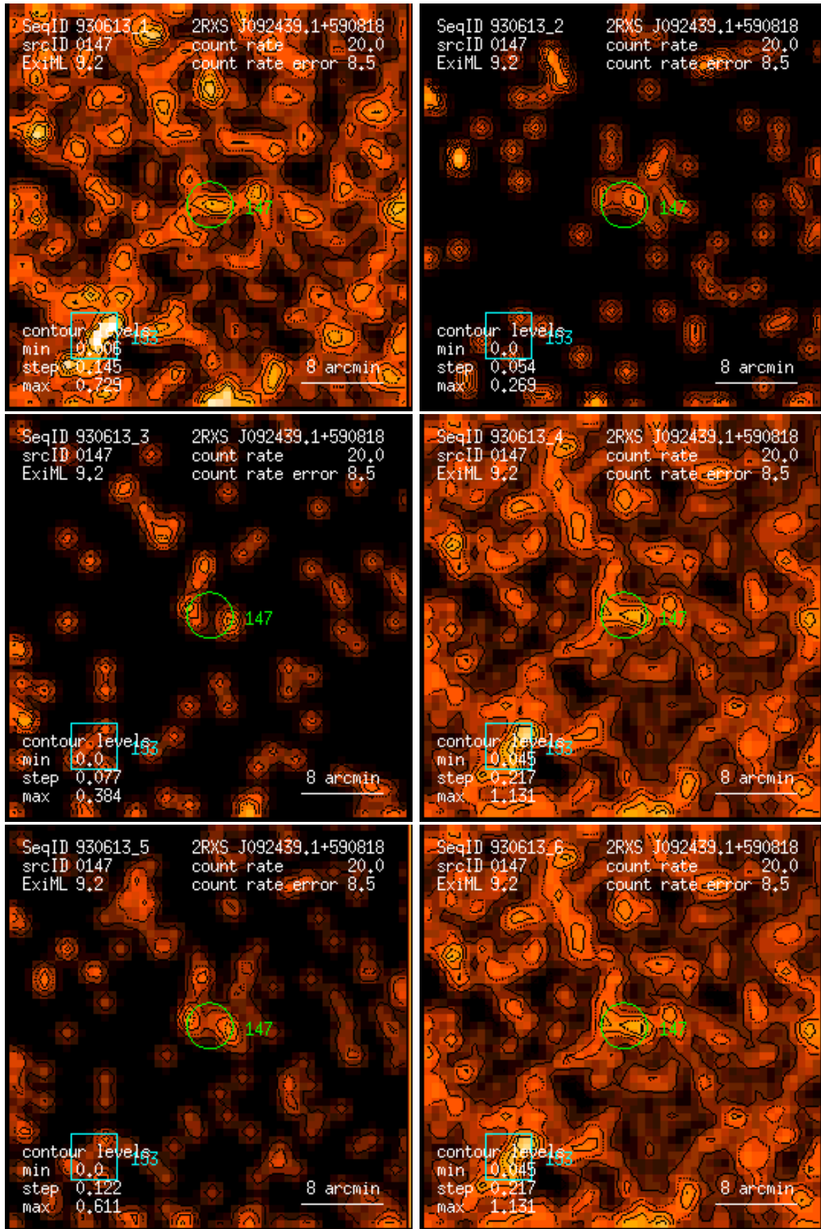
Figure 147: RASS 930613: detection 0147: band rate images, Gaussian filter: (1) PSPC channels 11 – 41, (2) 52 – 90, (3) 91 – 201, (4) 11 – 235, (5) 52 – 201, (6) 11 – 201. Broad band rates in counts/ks. Band rate contour levels in counts/ks/arcmin 2 .
