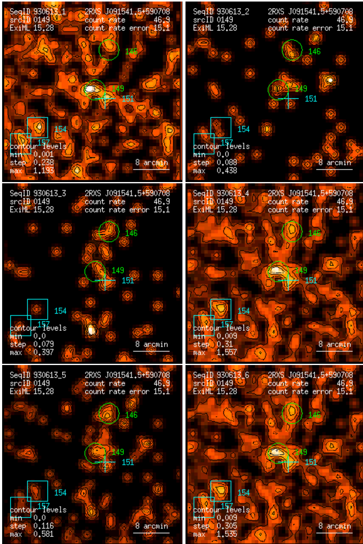
Figure 149: RASS 930613: detection 0149: band rate images, Gaussian filter: (1) PSPC channels 11 – 41, (2) 52 – 90, (3) 91 – 201, (4) 11 – 235, (5) 52 – 201, (6) 11 – 201. Broad band rates in counts/ks. Band rate contour levels in counts/ks/arcmin 2 .
