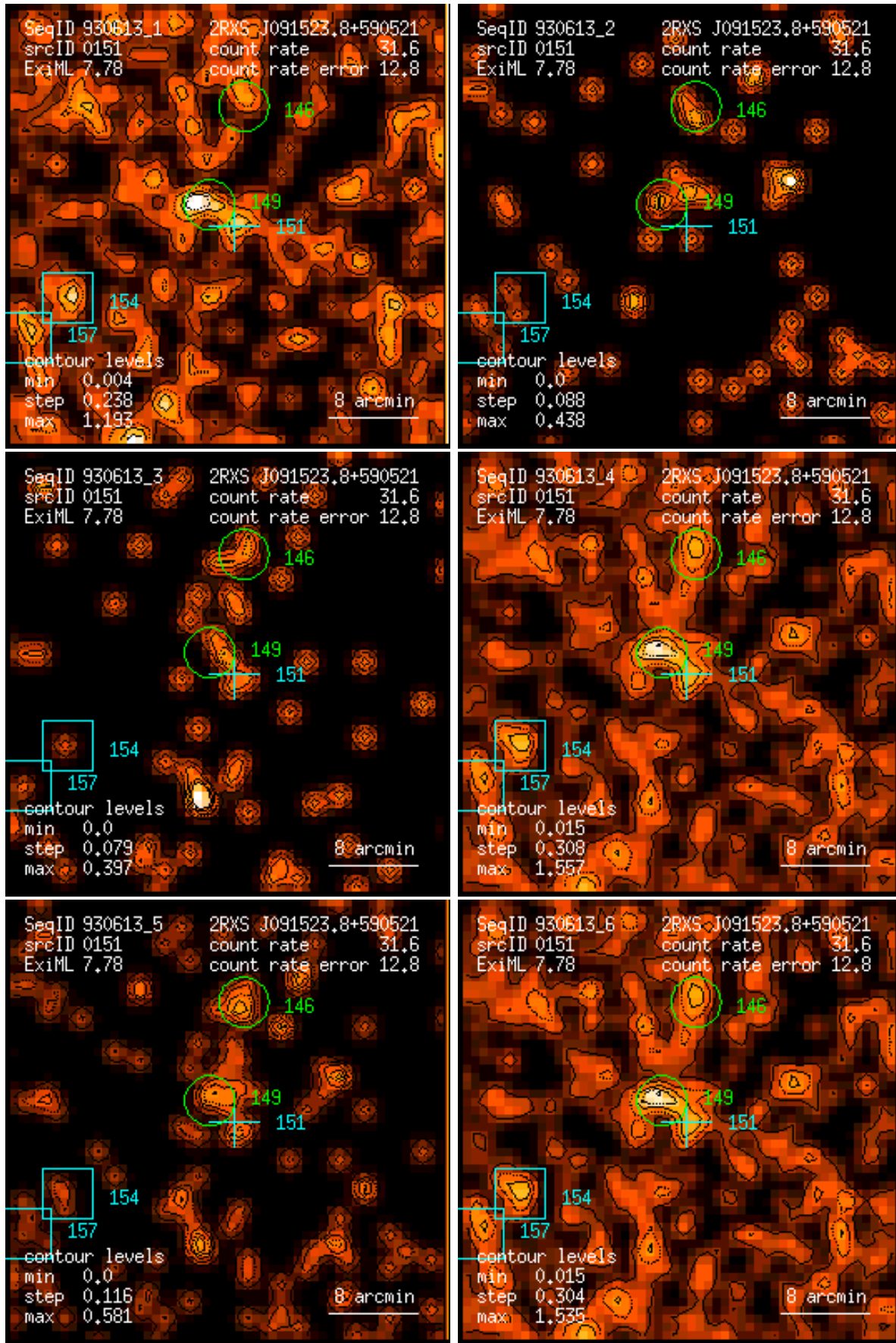
Figure 151: RASS 930613: detection 0151: band rate images, Gaussian filter: (1) PSPC channels 11 – 41, (2) 52 – 90, (3) 91 – 201, (4) 11 – 235, (5) 52 – 201, (6) 11 – 201. Broad band rates in counts/ks. Band rate contour levels in counts/ks/arcmin 2 .
