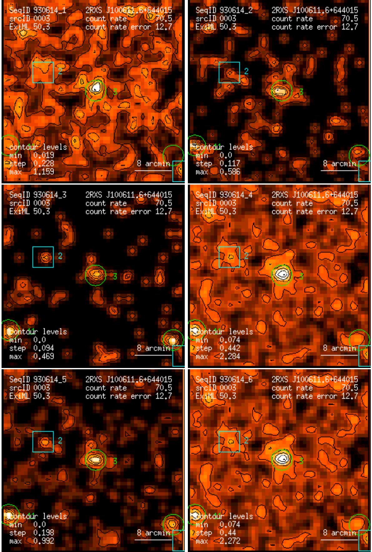
Figure 3: RASS 930614: detection 0003: band rate images, Gaussian filter: (1) PSPC channels 11 – 41, (2) 52 – 90, (3) 91 – 201, (4) 11 – 235, (5) 52 – 201, (6) 11 – 201. Broad band rates in counts/ks. Band rate contour levels in counts/ks/arcmin 2 .
