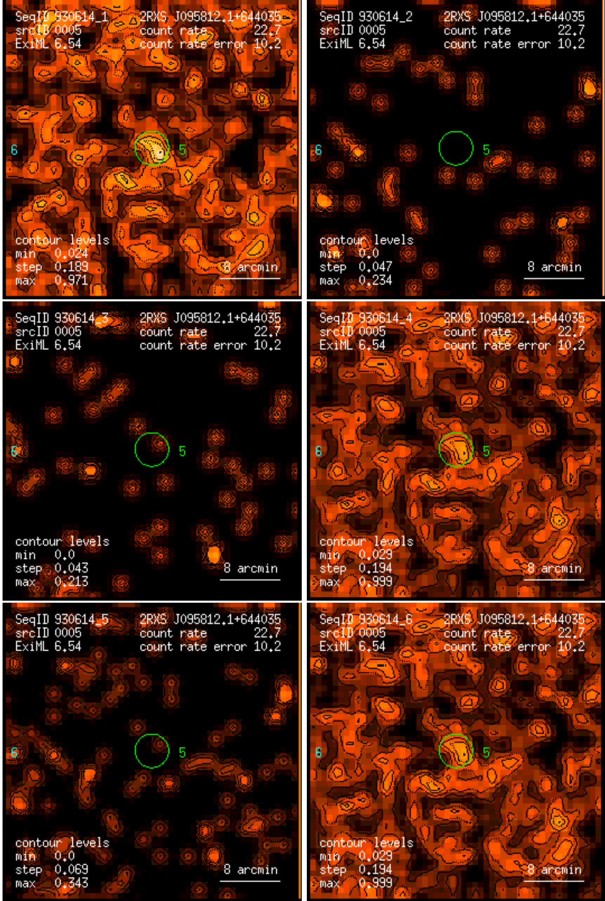
Figure 5: RASS 930614: detection 0005: band rate images, Gaussian filter: (1) PSPC channels 11 – 41, (2) 52 – 90, (3) 91 – 201, (4) 11 – 235, (5) 52 – 201, (6) 11 – 201. Broad band rates in counts/ks. Band rate contour levels in counts/ks/arcmin 2 .
