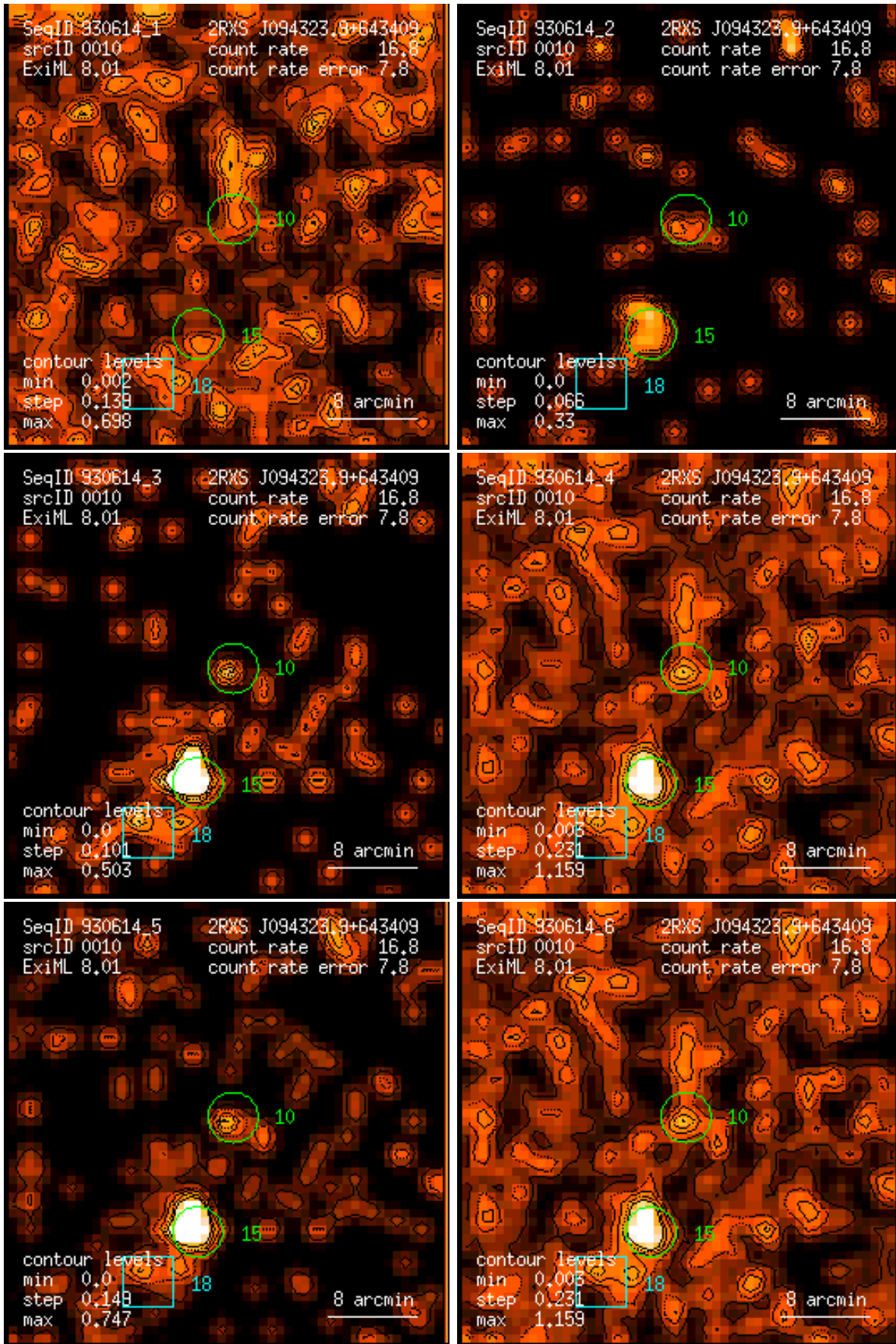
Figure 10: RASS 930614: detection 0010: band rate images, Gaussian filter: (1) PSPC channels 11 – 41, (2) 52 – 90, (3) 91 – 201, (4) 11 – 235, (5) 52 – 201, (6) 11 – 201. Broad band rates in counts/ks. Band rate contour levels in counts/ks/arcmin 2 .
