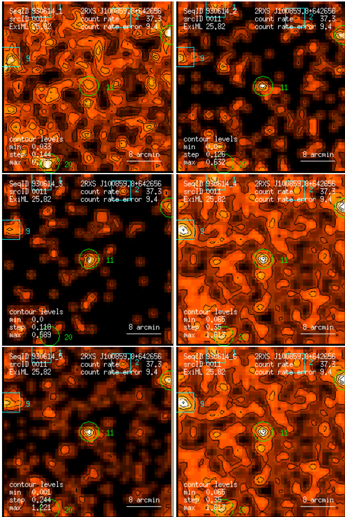
Figure 11: RASS 930614: detection 0011: band rate images, Gaussian filter: (1) PSPC channels 11 – 41, (2) 52 – 90, (3) 91 – 201, (4) 11 – 235, (5) 52 – 201, (6) 11 – 201. Broad band rates in counts/ks. Band rate contour levels in counts/ks/arcmin 2 .
