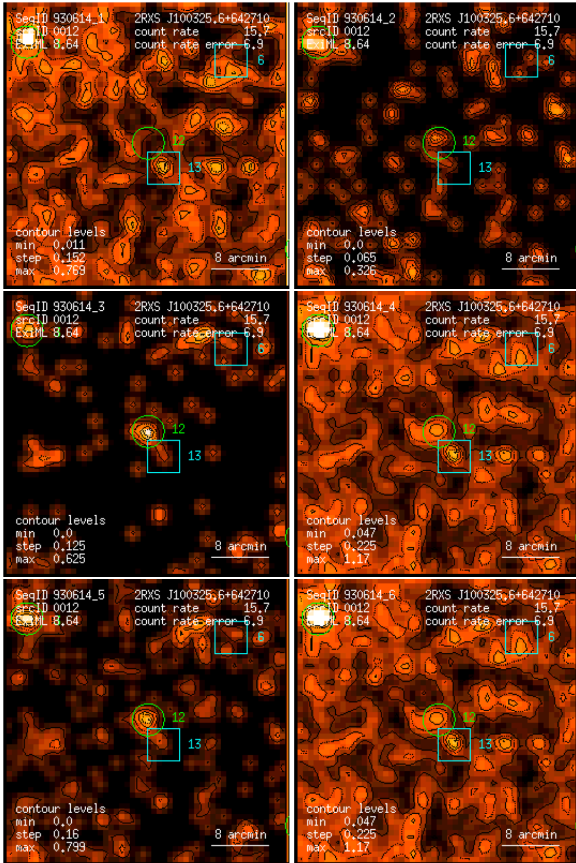
Figure 12: RASS 930614: detection 0012: band rate images, Gaussian filter: (1) PSPC channels 11 – 41, (2) 52 – 90, (3) 91 – 201, (4) 11 – 235, (5) 52 – 201, (6) 11 – 201. Broad band rates in counts/ks. Band rate contour levels in counts/ks/arcmin 2 .
