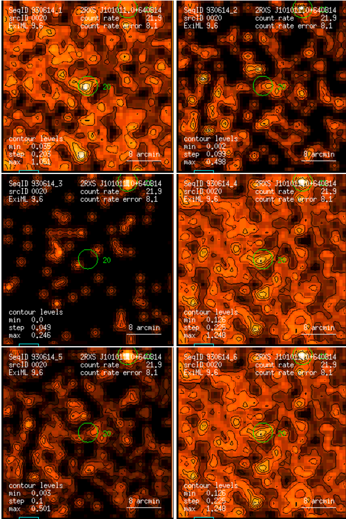
Figure 20: RASS 930614: detection 0020: band rate images, Gaussian filter: (1) PSPC channels 11 – 41, (2) 52 – 90, (3) 91 – 201, (4) 11 – 235, (5) 52 – 201, (6) 11 – 201. Broad band rates in counts/ks. Band rate contour levels in counts/ks/arcmin 2 .
