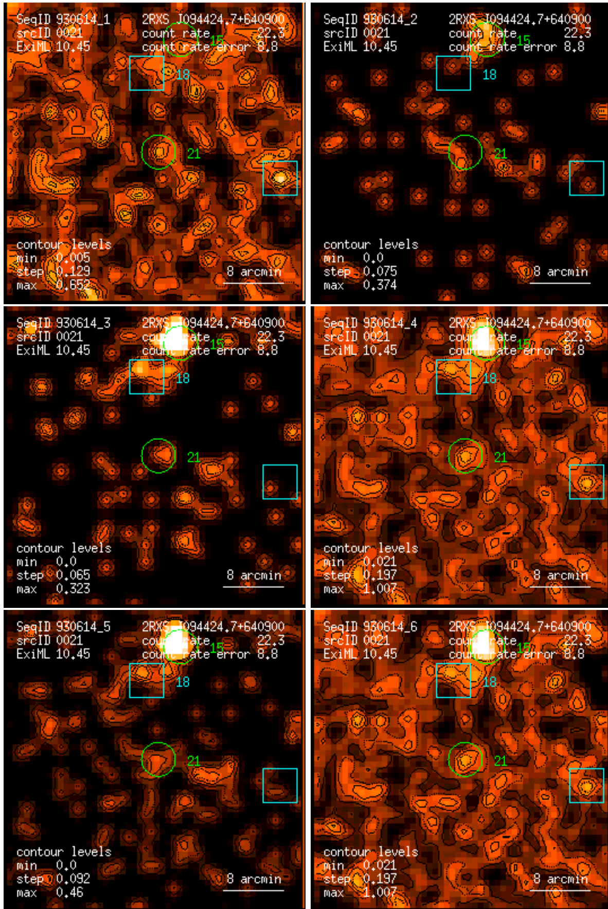
Figure 21: RASS 930614: detection 0021: band rate images, Gaussian filter: (1) PSPC channels 11 – 41, (2) 52 – 90, (3) 91 – 201, (4) 11 – 235, (5) 52 – 201, (6) 11 – 201. Broad band rates in counts/ks. Band rate contour levels in counts/ks/arcmin 2 .
