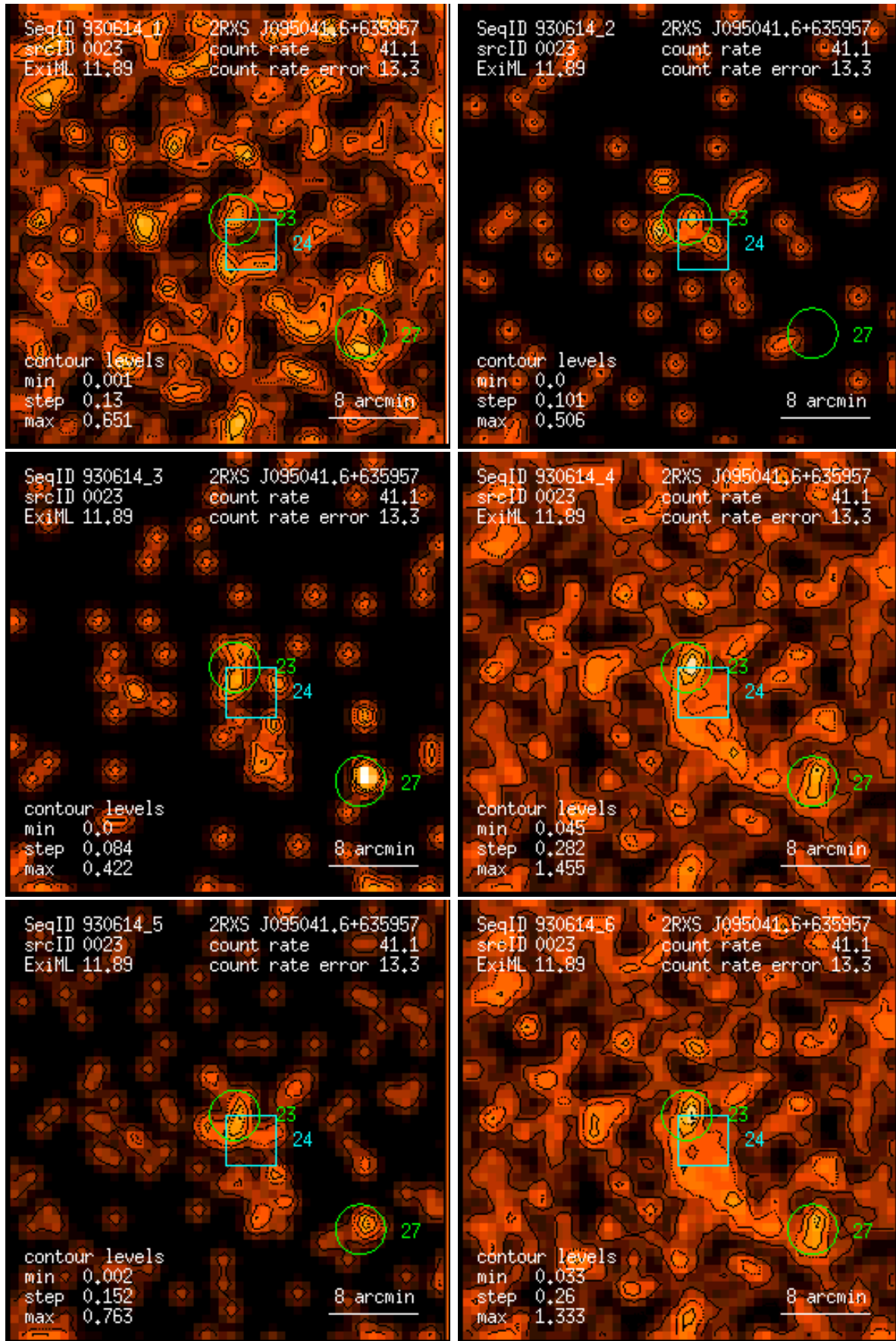
Figure 23: RASS 930614: detection 0023: band rate images, Gaussian filter: (1) PSPC channels 11 – 41, (2) 52 – 90, (3) 91 – 201, (4) 11 – 235, (5) 52 – 201, (6) 11 – 201. Broad band rates in counts/ks. Band rate contour levels in counts/ks/arcmin 2 .
