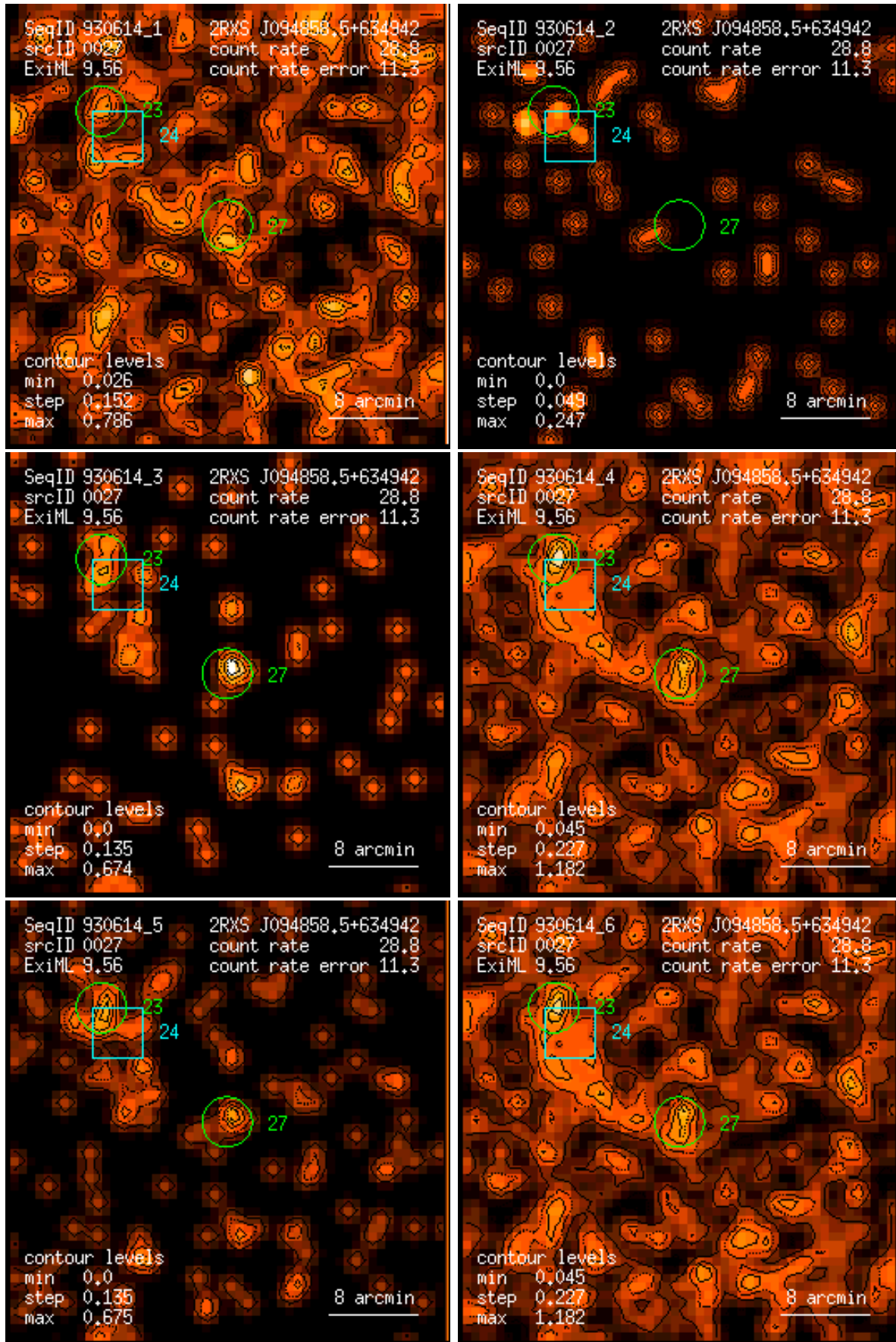
Figure 27: RASS 930614: detection 0027: band rate images, Gaussian filter: (1) PSPC channels 11 – 41, (2) 52 – 90, (3) 91 – 201, (4) 11 – 235, (5) 52 – 201, (6) 11 – 201. Broad band rates in counts/ks. Band rate contour levels in counts/ks/arcmin 2 .
