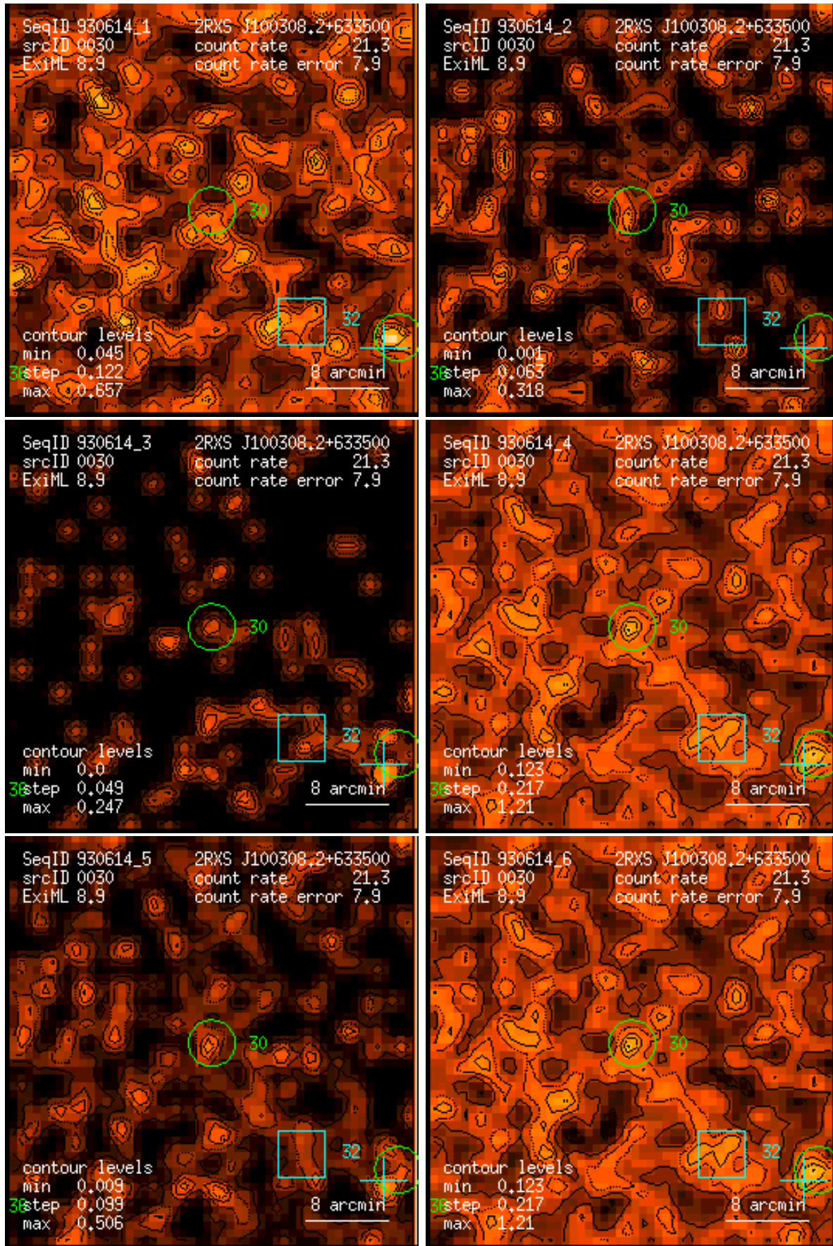
Figure 30: RASS 930614: detection 0030: band rate images, Gaussian filter: (1) PSPC channels 11 – 41, (2) 52 – 90, (3) 91 – 201, (4) 11 – 235, (5) 52 – 201, (6) 11 – 201. Broad band rates in counts/ks. Band rate contour levels in counts/ks/arcmin 2 .
