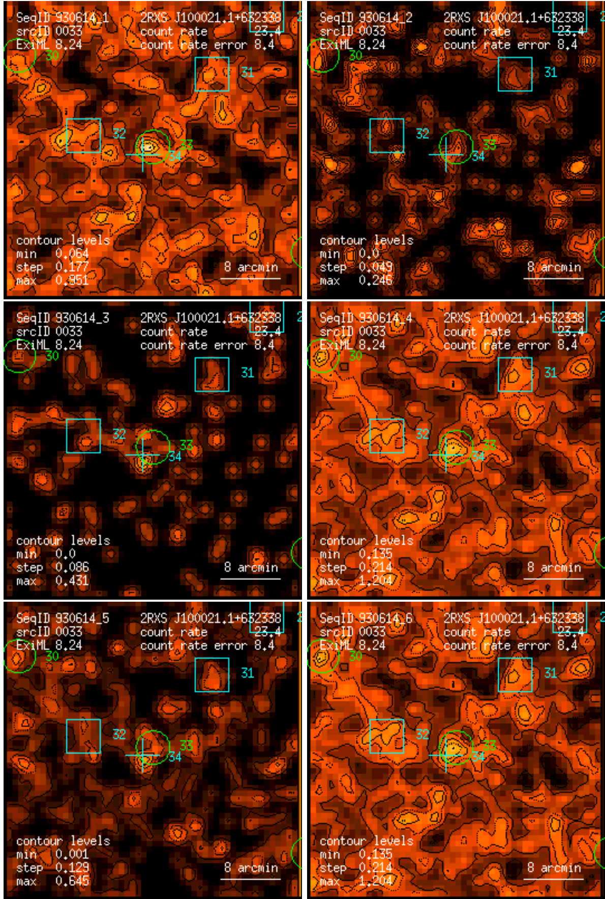
Figure 33: RASS 930614: detection 0033: band rate images, Gaussian filter: (1) PSPC channels 11 – 41, (2) 52 – 90, (3) 91 – 201, (4) 11 – 235, (5) 52 – 201, (6) 11 – 201. Broad band rates in counts/ks. Band rate contour levels in counts/ks/arcmin 2 .
