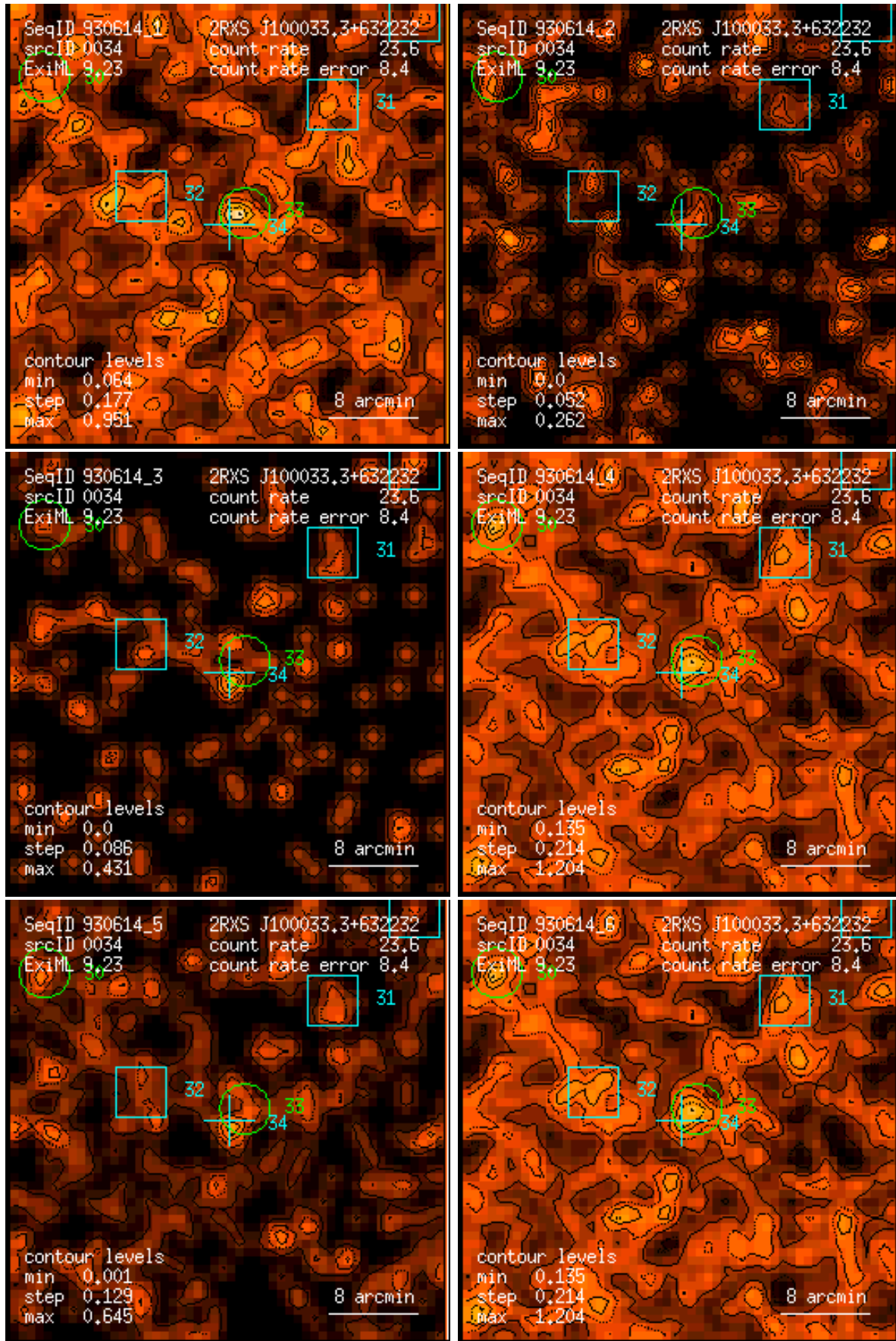
Figure 34: RASS 930614: detection 0034: band rate images, Gaussian filter: (1) PSPC channels 11 – 41, (2) 52 – 90, (3) 91 – 201, (4) 11 – 235, (5) 52 – 201, (6) 11 – 201. Broad band rates in counts/ks. Band rate contour levels in counts/ks/arcmin 2 .
