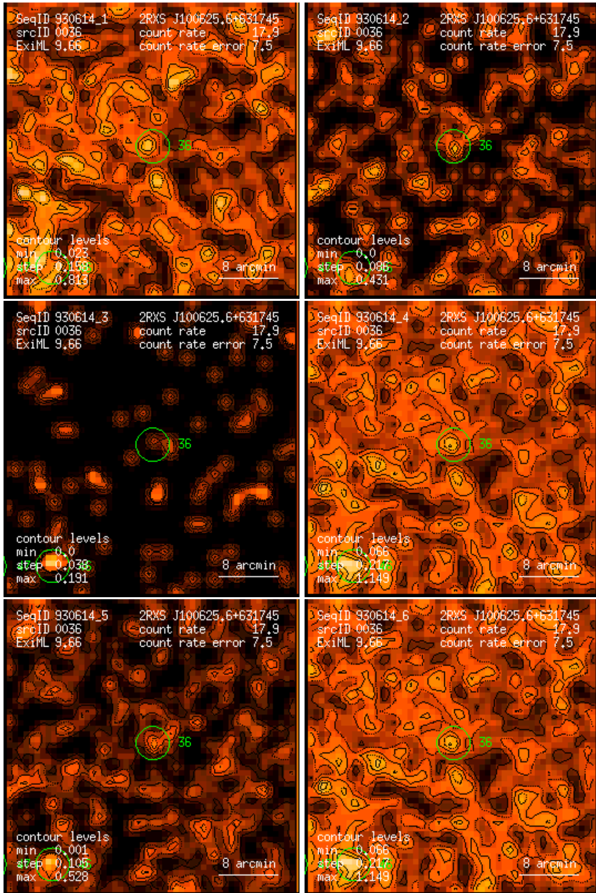
Figure 36: RASS 930614: detection 0036: band rate images, Gaussian filter: (1) PSPC channels 11 – 41, (2) 52 – 90, (3) 91 – 201, (4) 11 – 235, (5) 52 – 201, (6) 11 – 201. Broad band rates in counts/ks. Band rate contour levels in counts/ks/arcmin 2 .
