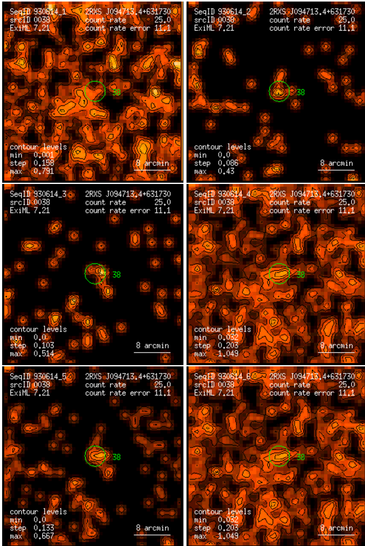
Figure 38: RASS 930614: detection 0038: band rate images, Gaussian filter: (1) PSPC channels 11 – 41, (2) 52 – 90, (3) 91 – 201, (4) 11 – 235, (5) 52 – 201, (6) 11 – 201. Broad band rates in counts/ks. Band rate contour levels in counts/ks/arcmin 2 .
