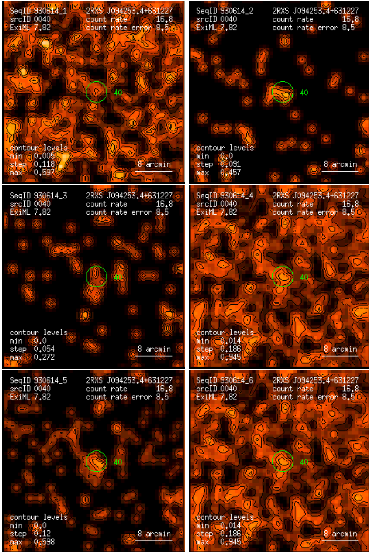
Figure 40: RASS 930614: detection 0040: band rate images, Gaussian filter: (1) PSPC channels 11 – 41, (2) 52 – 90, (3) 91 – 201, (4) 11 – 235, (5) 52 – 201, (6) 11 – 201. Broad band rates in counts/ks. Band rate contour levels in counts/ks/arcmin 2 .
