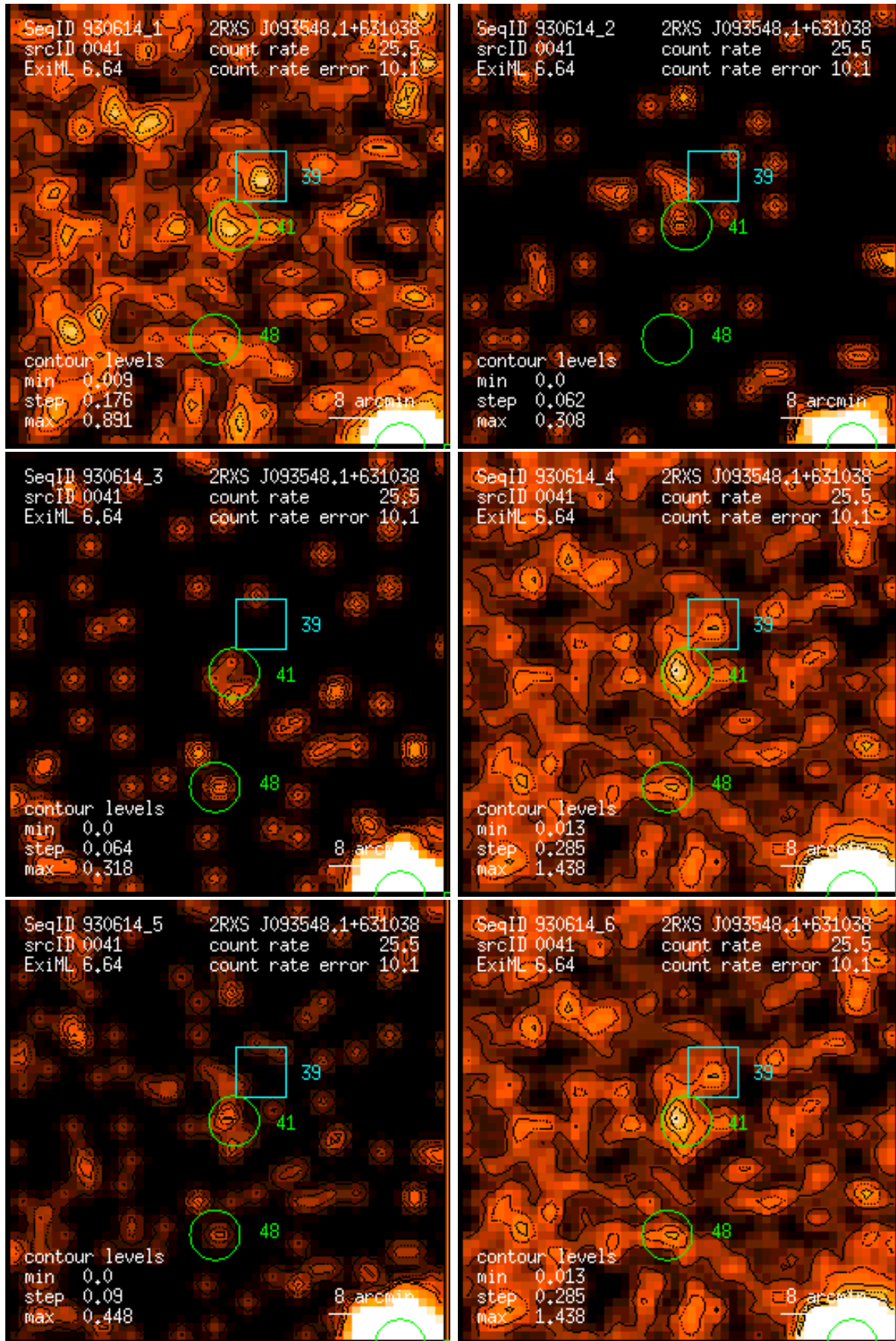
Figure 41: RASS 930614: detection 0041: band rate images, Gaussian filter: (1) PSPC channels 11 – 41, (2) 52 – 90, (3) 91 – 201, (4) 11 – 235, (5) 52 – 201, (6) 11 – 201. Broad band rates in counts/ks. Band rate contour levels in counts/ks/arcmin 2 .
