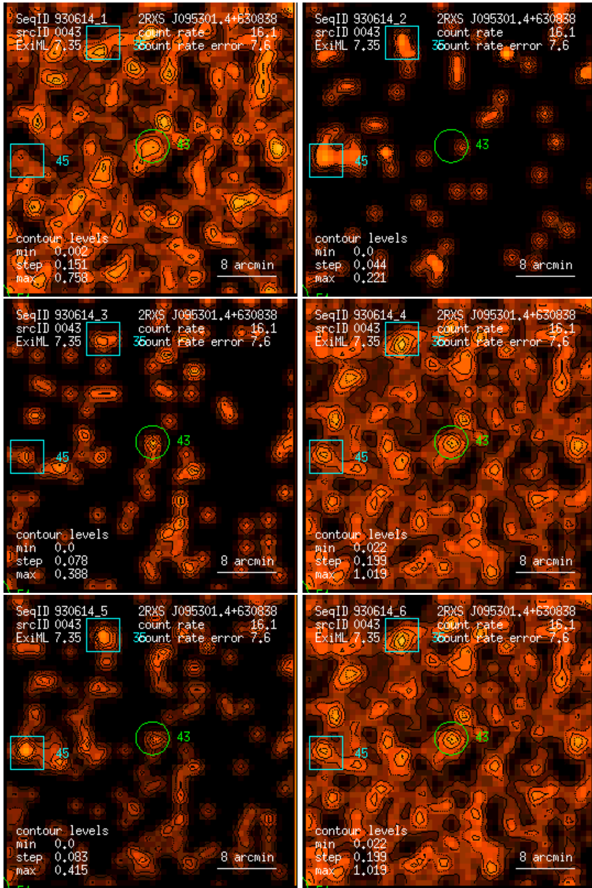
Figure 43: RASS 930614: detection 0043: band rate images, Gaussian filter: (1) PSPC channels 11 – 41, (2) 52 – 90, (3) 91 – 201, (4) 11 – 235, (5) 52 – 201, (6) 11 – 201. Broad band rates in counts/ks. Band rate contour levels in counts/ks/arcmin 2 .
