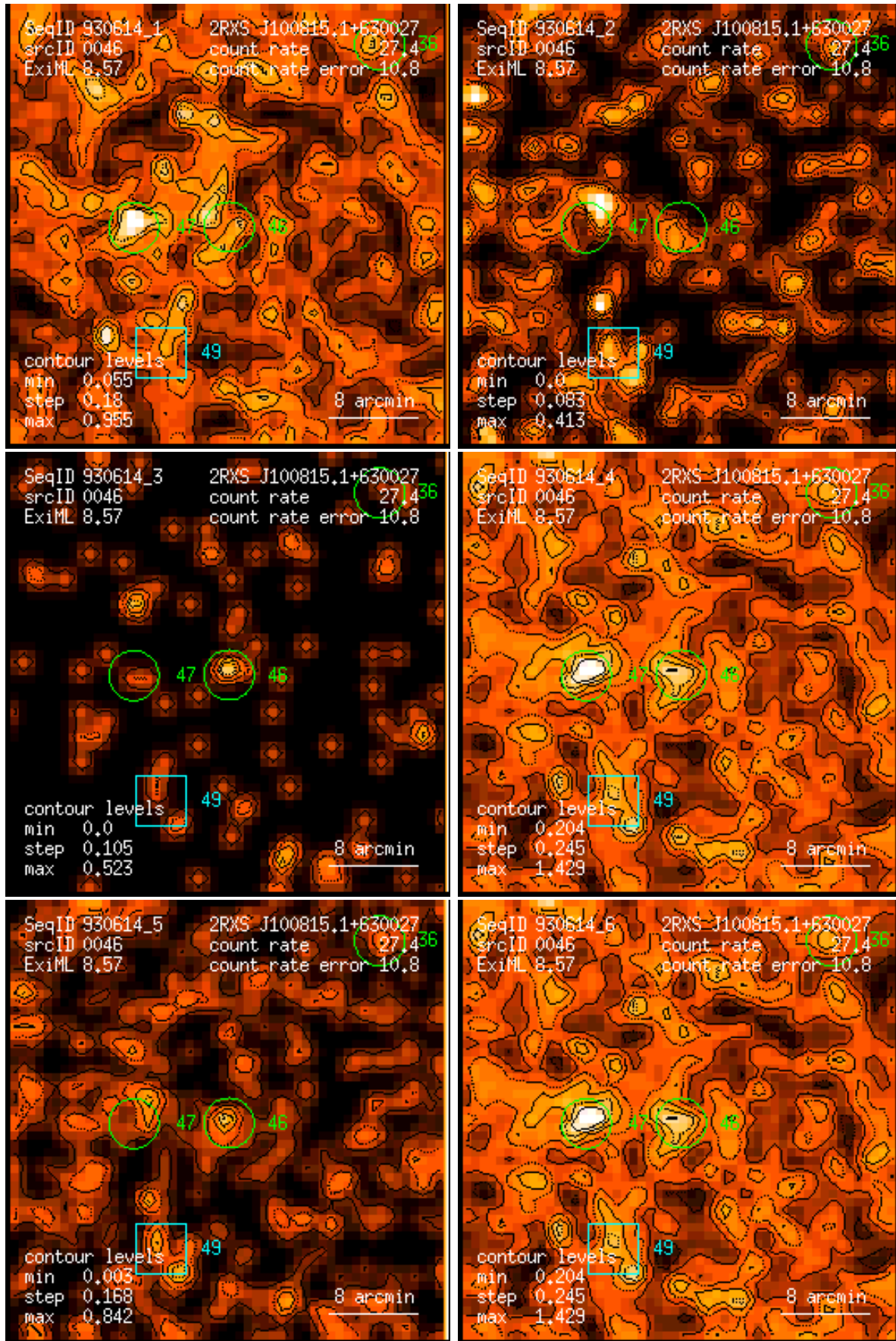
Figure 46: RASS 930614: detection 0046: band rate images, Gaussian filter: (1) PSPC channels 11 – 41, (2) 52 – 90, (3) 91 – 201, (4) 11 – 235, (5) 52 – 201, (6) 11 – 201. Broad band rates in counts/ks. Band rate contour levels in counts/ks/arcmin 2 .
