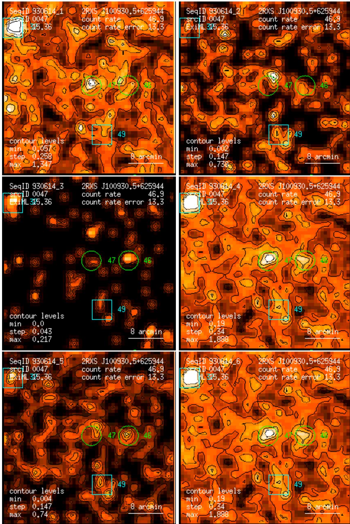
Figure 47: RASS 930614: detection 0047: band rate images, Gaussian filter: (1) PSPC channels 11 – 41, (2) 52 – 90, (3) 91 – 201, (4) 11 – 235, (5) 52 – 201, (6) 11 – 201. Broad band rates in counts/ks. Band rate contour levels in counts/ks/arcmin 2 .
