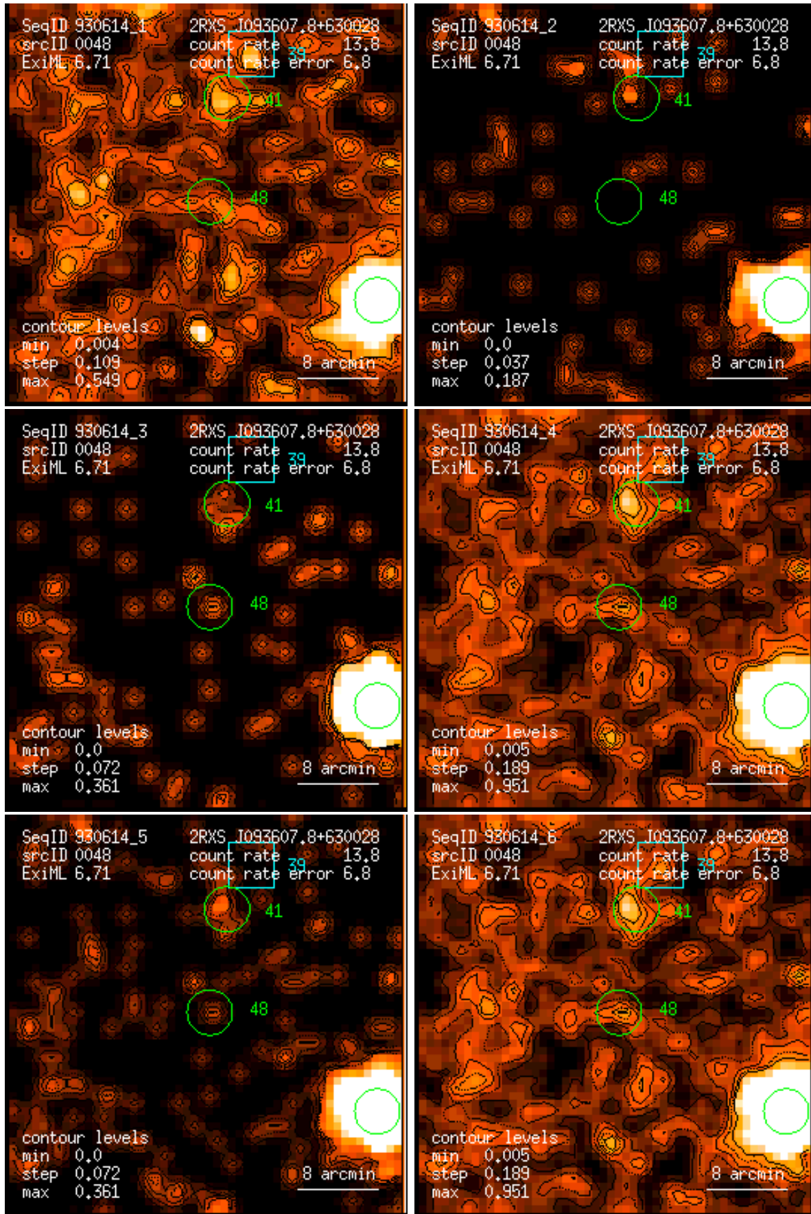
Figure 48: RASS 930614: detection 0048: band rate images, Gaussian filter: (1) PSPC channels 11 – 41, (2) 52 – 90, (3) 91 – 201, (4) 11 – 235, (5) 52 – 201, (6) 11 – 201. Broad band rates in counts/ks. Band rate contour levels in counts/ks/arcmin 2 .
