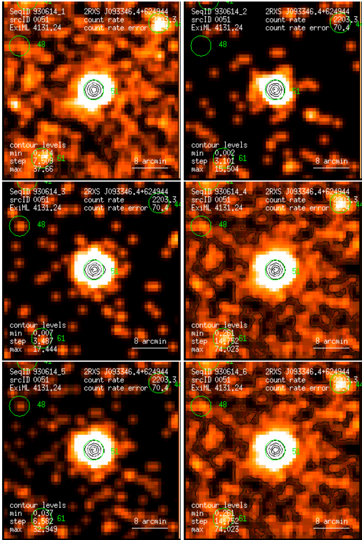
Figure 51: RASS 930614: detection 0051: band rate images, Gaussian filter: (1) PSPC channels 11 – 41, (2) 52 – 90, (3) 91 – 201, (4) 11 – 235, (5) 52 – 201, (6) 11 – 201. Broad band rates in counts/ks. Band rate contour levels in counts/ks/arcmin 2 .
