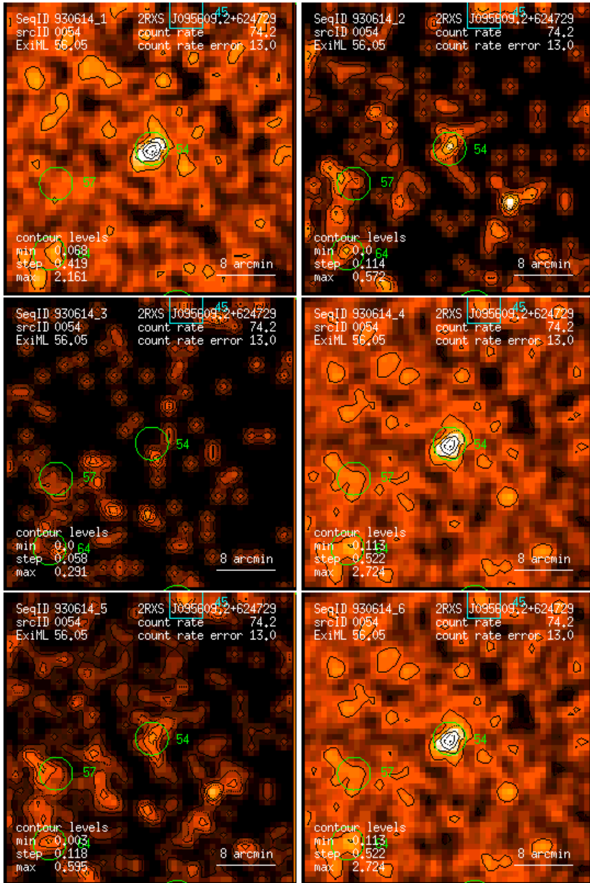
Figure 54: RASS 930614: detection 0054: band rate images, Gaussian filter: (1) PSPC channels 11 – 41, (2) 52 – 90, (3) 91 – 201, (4) 11 – 235, (5) 52 – 201, (6) 11 – 201. Broad band rates in counts/ks. Band rate contour levels in counts/ks/arcmin 2 .
