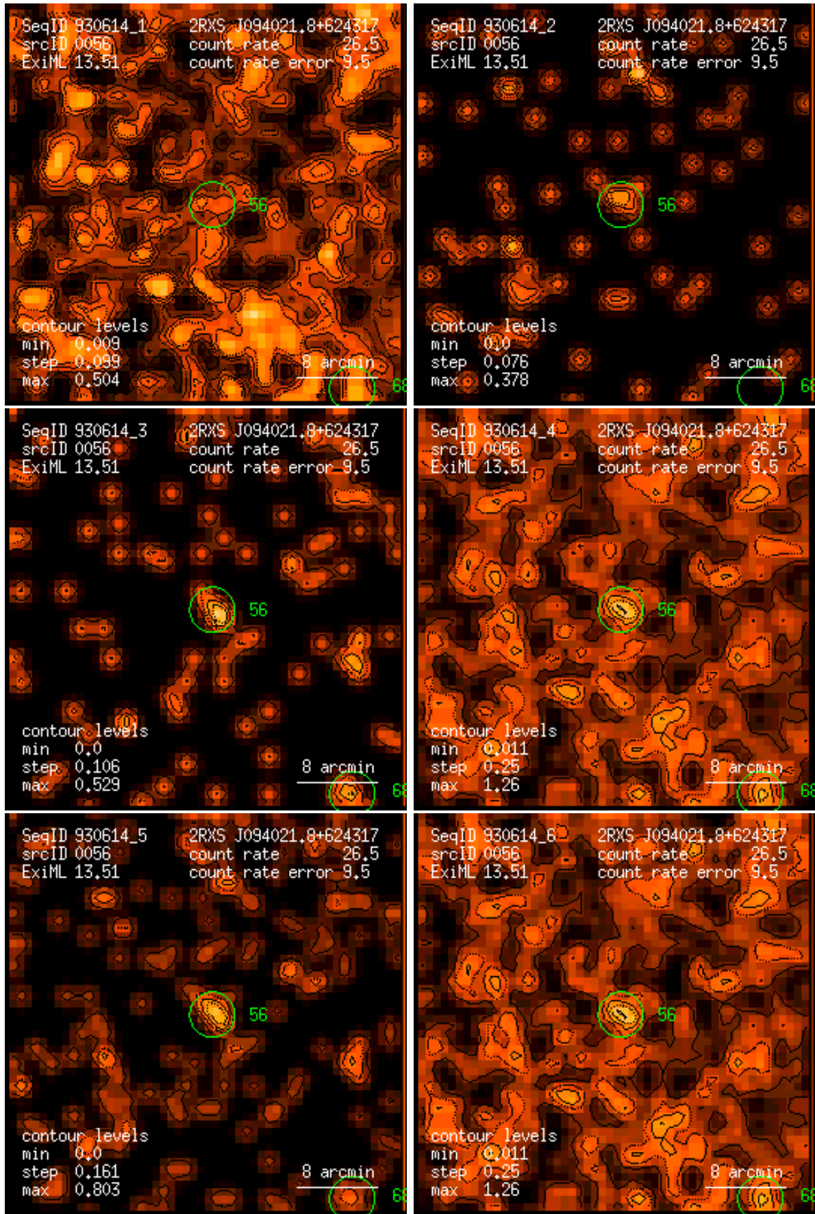
Figure 56: RASS 930614: detection 0056: band rate images, Gaussian filter: (1) PSPC channels 11 – 41, (2) 52 – 90, (3) 91 – 201, (4) 11 – 235, (5) 52 – 201, (6) 11 – 201. Broad band rates in counts/ks. Band rate contour levels in counts/ks/arcmin 2 .
