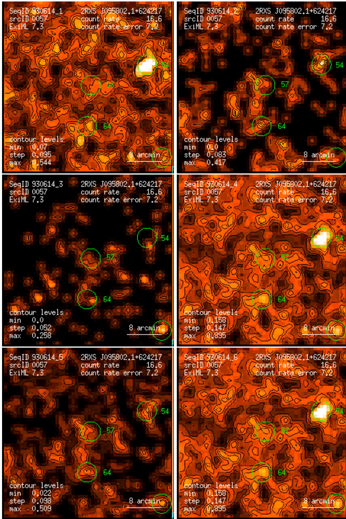
Figure 57: RASS 930614: detection 0057: band rate images, Gaussian filter: (1) PSPC channels 11 – 41, (2) 52 – 90, (3) 91 – 201, (4) 11 – 235, (5) 52 – 201, (6) 11 – 201. Broad band rates in counts/ks. Band rate contour levels in counts/ks/arcmin 2 .
