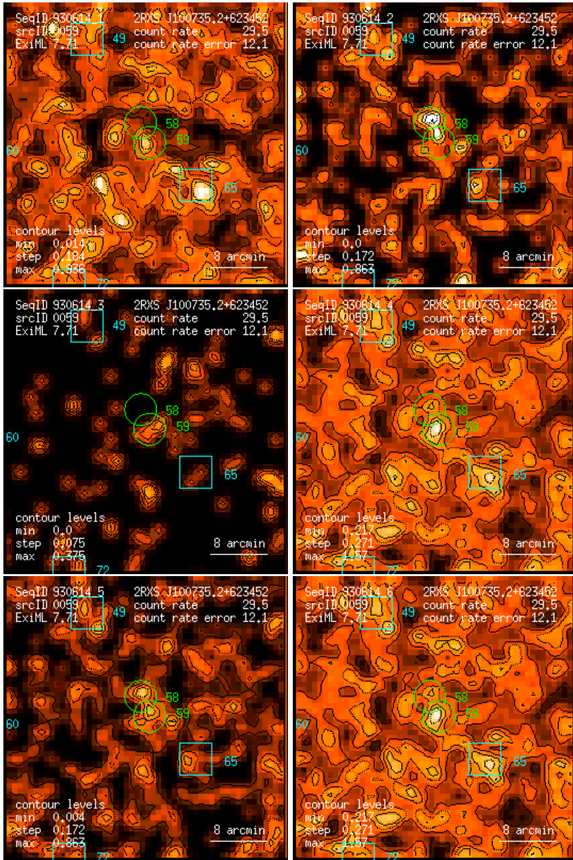
Figure 59: RASS 930614: detection 0059: band rate images, Gaussian filter: (1) PSPC channels 11 – 41, (2) 52 – 90, (3) 91 – 201, (4) 11 – 235, (5) 52 – 201, (6) 11 – 201. Broad band rates in counts/ks. Band rate contour levels in counts/ks/arcmin 2 .
