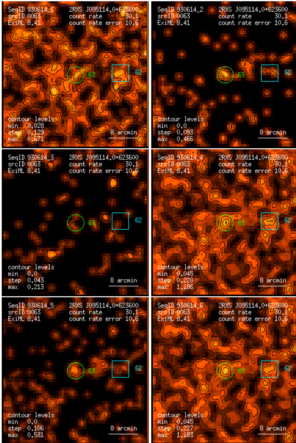
Figure 63: RASS 930614: detection 0063: band rate images, Gaussian filter: (1) PSPC channels 11 – 41, (2) 52 – 90, (3) 91 – 201, (4) 11 – 235, (5) 52 – 201, (6) 11 – 201. Broad band rates in counts/ks. Band rate contour levels in counts/ks/arcmin 2 .
