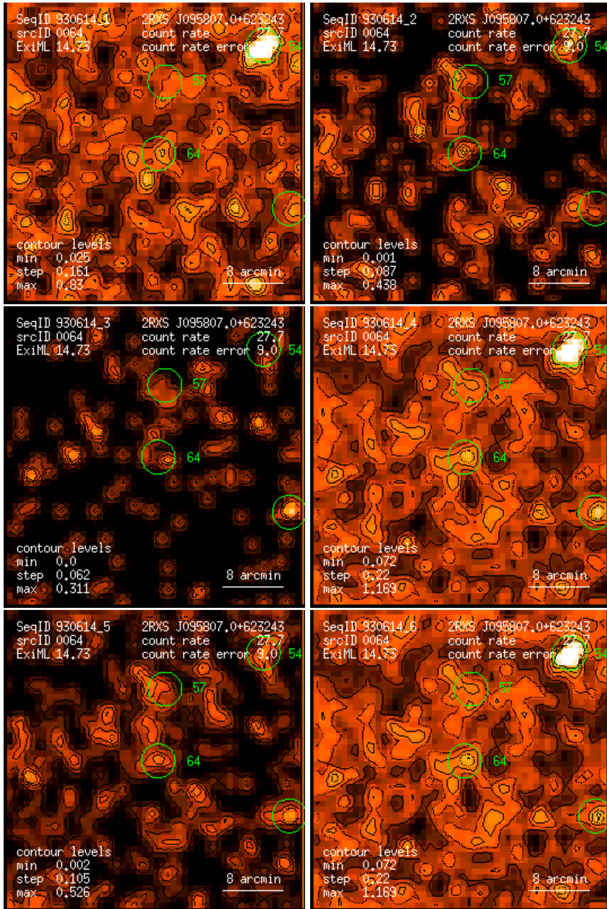
Figure 64: RASS 930614: detection 0064: band rate images, Gaussian filter: (1) PSPC channels 11 – 41, (2) 52 – 90, (3) 91 – 201, (4) 11 – 235, (5) 52 – 201, (6) 11 – 201. Broad band rates in counts/ks. Band rate contour levels in counts/ks/arcmin 2 .
