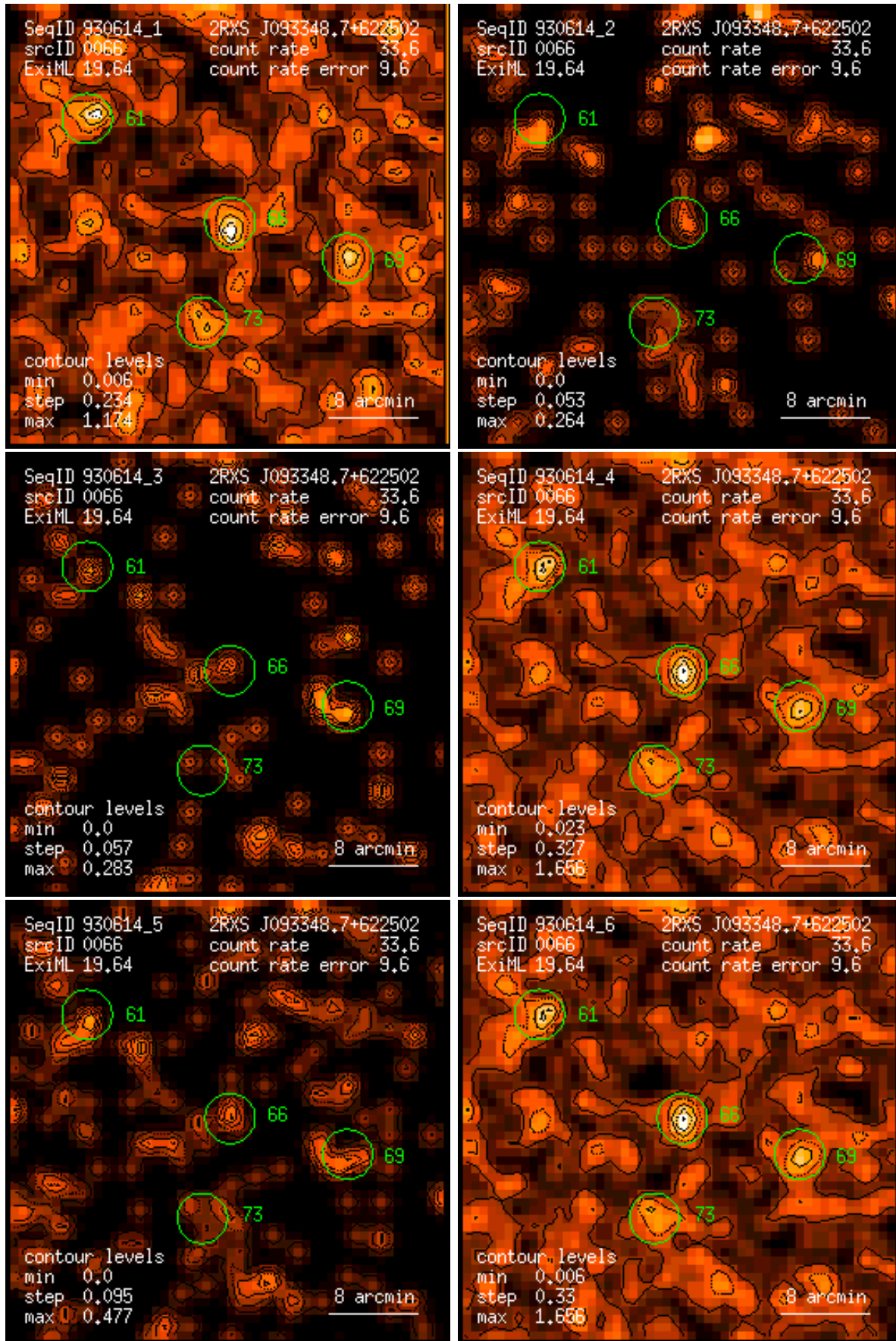
Figure 66: RASS 930614: detection 0066: band rate images, Gaussian filter: (1) PSPC channels 11 – 41, (2) 52 – 90, (3) 91 – 201, (4) 11 – 235, (5) 52 – 201, (6) 11 – 201. Broad band rates in counts/ks. Band rate contour levels in counts/ks/arcmin 2 .
