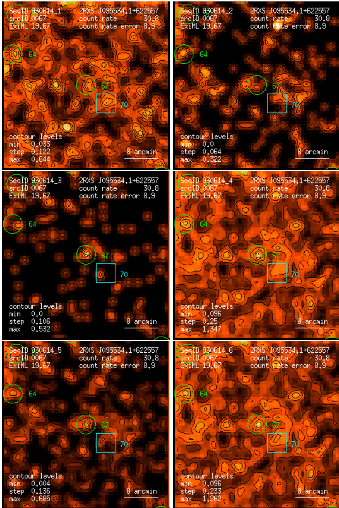
Figure 67: RASS 930614: detection 0067: band rate images, Gaussian filter: (1) PSPC channels 11 – 41, (2) 52 – 90, (3) 91 – 201, (4) 11 – 235, (5) 52 – 201, (6) 11 – 201. Broad band rates in counts/ks. Band rate contour levels in counts/ks/arcmin 2 .
