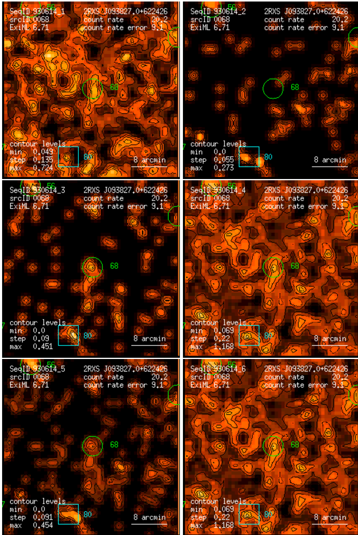
Figure 68: RASS 930614: detection 0068: band rate images, Gaussian filter: (1) PSPC channels 11 – 41, (2) 52 – 90, (3) 91 – 201, (4) 11 – 235, (5) 52 – 201, (6) 11 – 201. Broad band rates in counts/ks. Band rate contour levels in counts/ks/arcmin 2 .
