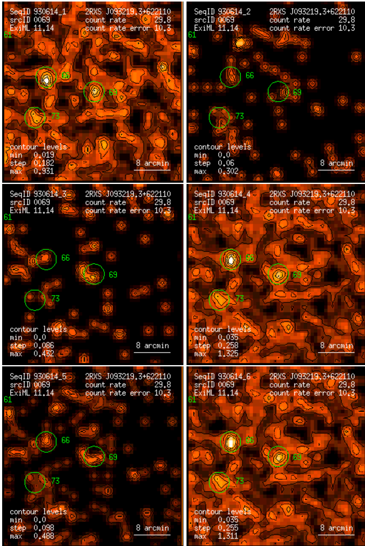
Figure 69: RASS 930614: detection 0069: band rate images, Gaussian filter: (1) PSPC channels 11 – 41, (2) 52 – 90, (3) 91 – 201, (4) 11 – 235, (5) 52 – 201, (6) 11 – 201. Broad band rates in counts/ks. Band rate contour levels in counts/ks/arcmin 2 .
