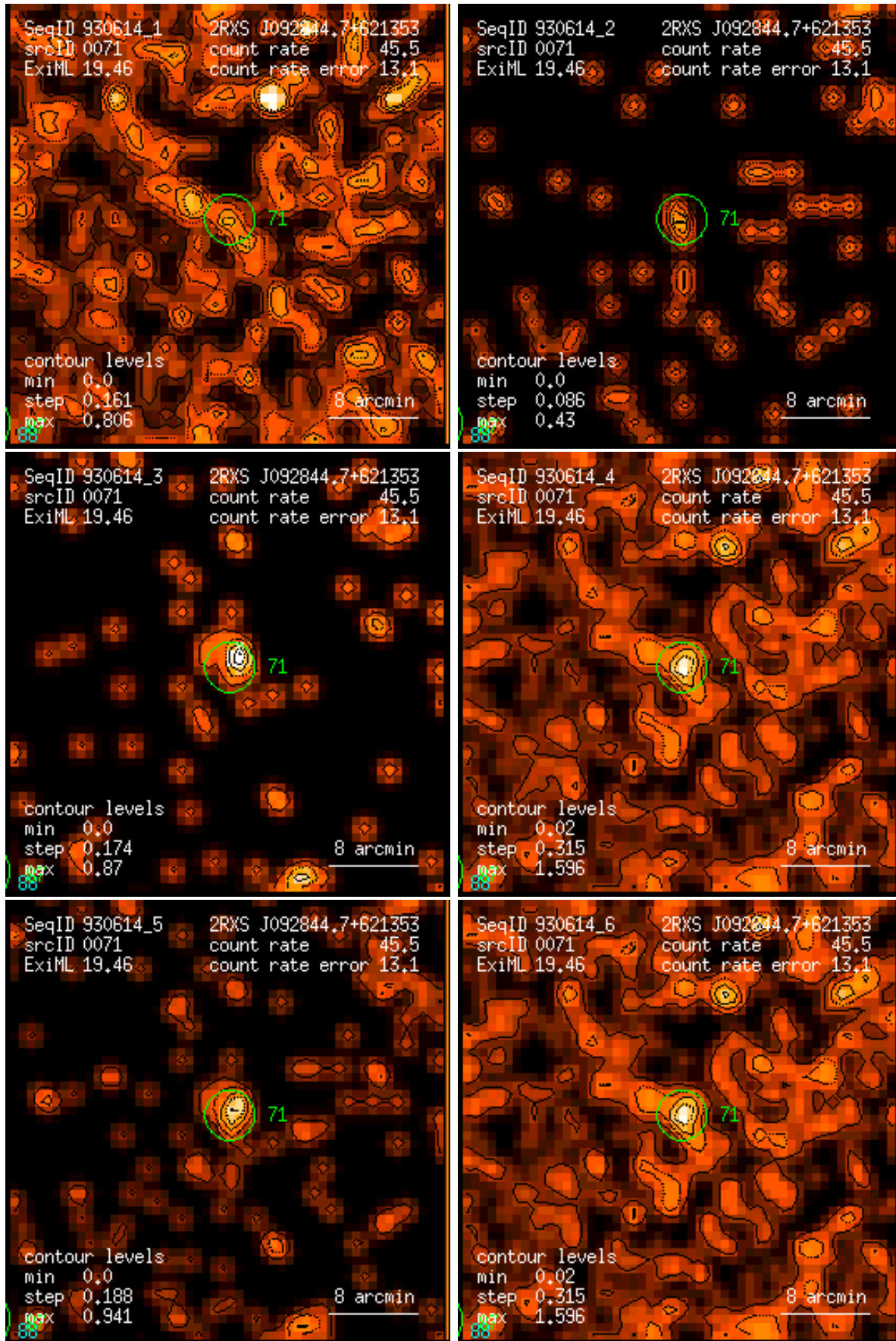
Figure 71: RASS 930614: detection 0071: band rate images, Gaussian filter: (1) PSPC channels 11 – 41, (2) 52 – 90, (3) 91 – 201, (4) 11 – 235, (5) 52 – 201, (6) 11 – 201. Broad band rates in counts/ks. Band rate contour levels in counts/ks/arcmin 2 .
