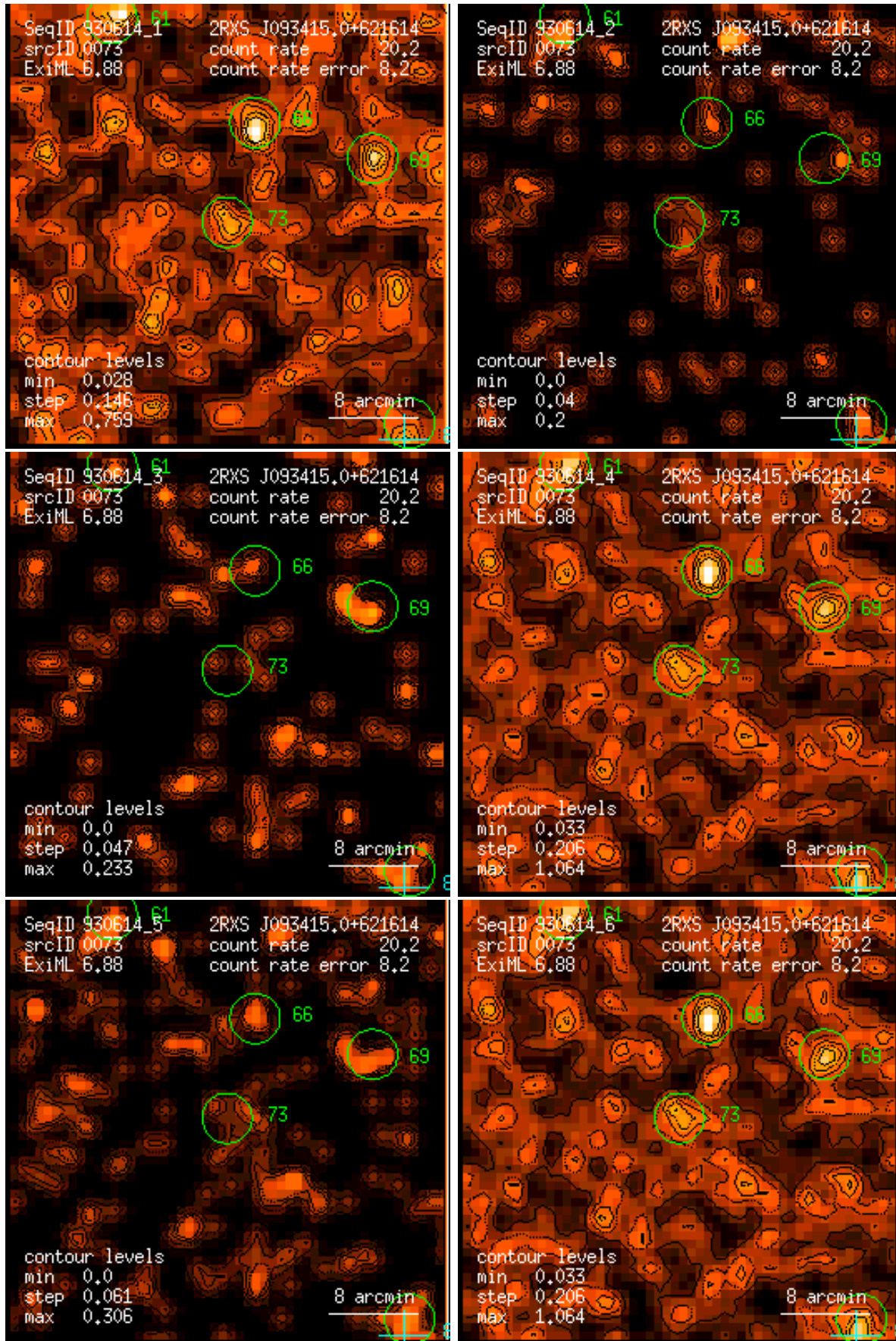
Figure 73: RASS 930614: detection 0073: band rate images, Gaussian filter: (1) PSPC channels 11 – 41, (2) 52 – 90, (3) 91 – 201, (4) 11 – 235, (5) 52 – 201, (6) 11 – 201. Broad band rates in counts/ks. Band rate contour levels in counts/ks/arcmin 2 .
